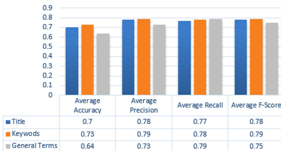
Figure 14. ACM (individual metadata).
