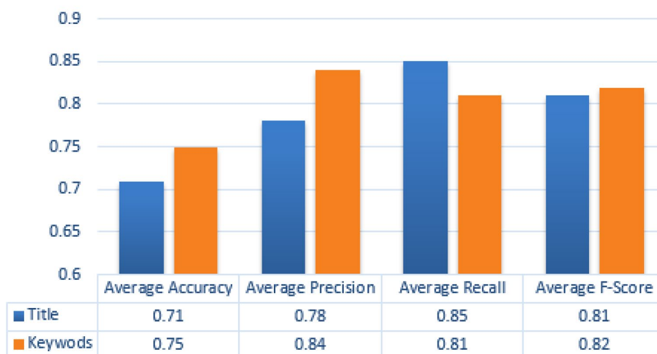
Figure 13. JUCS (individual metadata).
