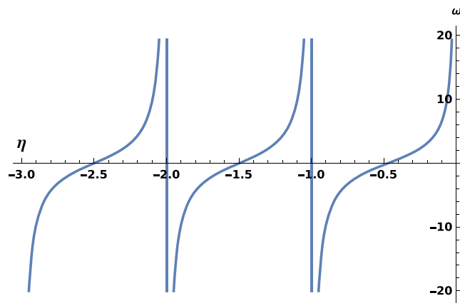
Figure 8. \omega versus \eta in the attractive case.
