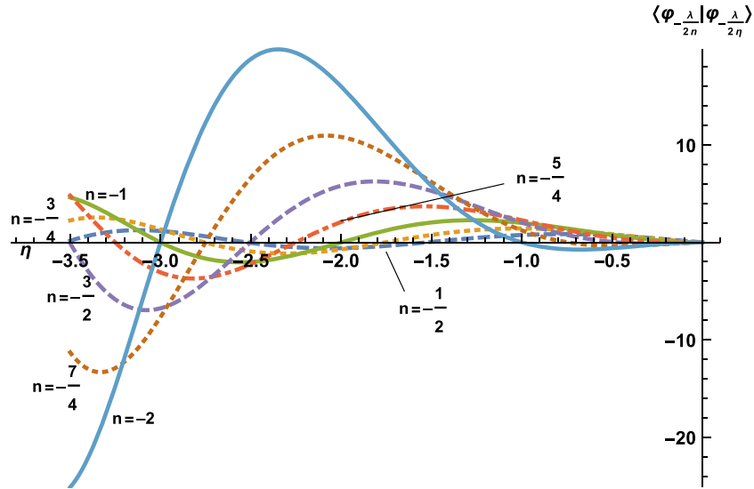
Figure 1. Here are the curves \eta \mapsto \langle \varphi_{\frac{\lambda}{2n}} | \varphi_{\frac{\lambda}{2n}} \rangle , for n = -1/2 (dashed line), n = -3/4 (dotted line), n = -1 (plain line), n = -5/4 (dot-dashed line), n = -3/2 (dashed line), n = -7/4 (dotted line) and n = -2 (plain line). The zeros of each curve read \eta = \frac{\lambda}{2\sqrt{-e}} where e \in \mathcal{S}_\omega , with \omega = -g_b(n) , as explained further on. The curves seem to form pairs corresponding to (n, n + 1) , in particular, one could believe that each pair intersects on the \eta -axis (abscissa), but this is wrong, except for (n, n + 1) = (-2, -1) which correspond to the same Rydberg set \mathcal{S}_\infty . All the other intersections are only close to zero, so that, indeed, \mathcal{S}_{-g_b(n)} \neq \mathcal{S}_{-g_b(n+1)} . \eta = n is missing, because \langle \varphi_{\frac{\lambda}{2n}} | \varphi_{\frac{\lambda}{2n}} \rangle \neq 0 .
