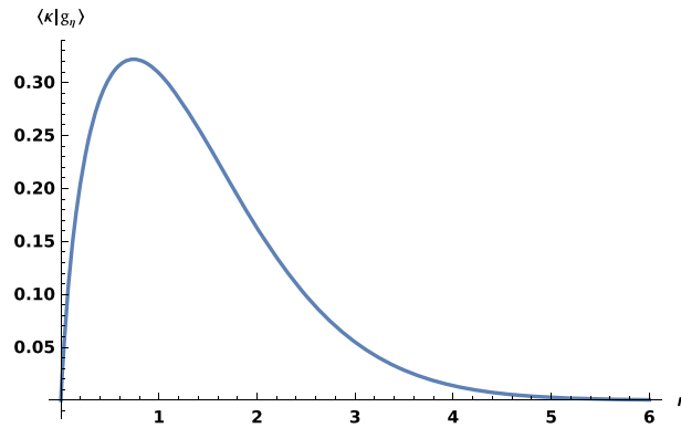
Figure 5. \langle \kappa | g_\eta \rangle versus \eta .
