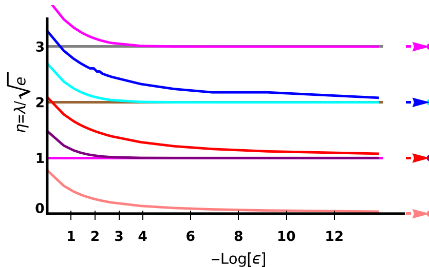
Figure 7. First energies of \frac{p^2}{2m} + V_\epsilon(e_1^\epsilon, e_2^\epsilon, e_3^\epsilon, e_4^\epsilon, e_5^\epsilon) and e_3^\epsilon from bottom to top) versus \ln(1/\epsilon) in dimensionless y-scale. The asymptotic limit is indicated by an arrow on the right, for each curve and by the horizontal straight lines.
