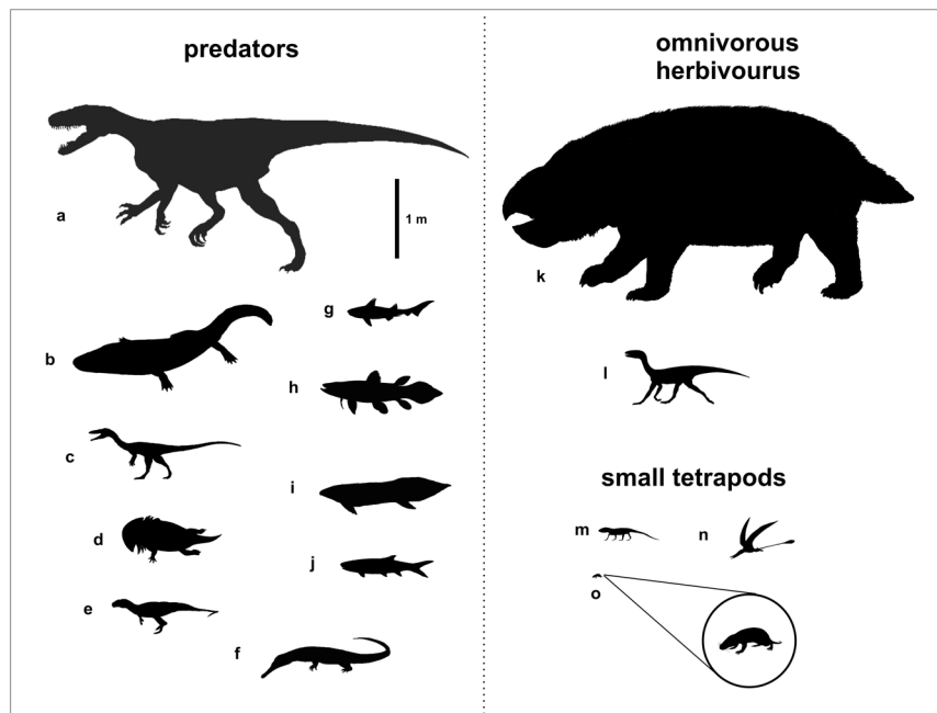
Figure 2. Sketch-drawing of the vertebrate faunal assemblage of the Lisowice site (modified from Niedźwiedzki 10 ). (a) Large, theropod-like predatory archosaur ( Smok wawelski ); (b) large temnospondyl amphibian ( Cyclotosaurus sp.); (c) small predatory dinosaurs (Neotheropoda indet.); (d) temnospondyl amphibian ( Gerrothorax sp.); (e) small basal crocodylomorph (Crocodylomorpha indet.); (f) small diapsid (Choristodere-like animal); (g) hybodont sharks ( Polyacrodus and Hybodus ); (h) coelacanth fish; (i) dipnoan fish ( Ptychoceratodus sp.); (j) actinopterygian fish; (k) gigantic dicynodont; (l) dinosauriforms or early dinosaurs (Dinosauriformes indet. or Dinosauria indet.); (m) small lepidosauromorphs (Sphenodontia indet.); (n) pterosaurs (Pterosauria indet.); (o) early mammaliaform ( Hallautherium sp.).
