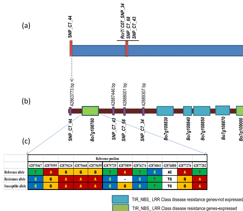
Figure 3. Rcr7 location on chromosome C7. (a) Genetic location of Rcr7 . (b) Physical locations of the SNP markers and TIR-NBS-LRR disease resistance genes in the Rcr7 target region. The length of the boxes reflects the sizes of the genes. (c) Comparison of polymorphic variants at the Bo7g108760 loci between the reference genome, R pool and S pool.
