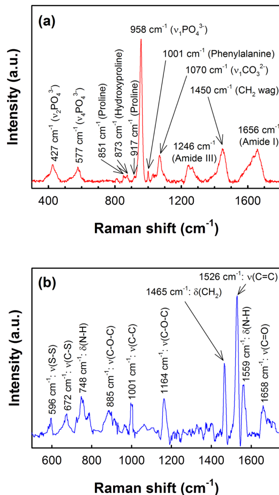
Figure 1. Typical Raman spectrum of (a) healthy human bone and (b) S. aureus bacteria obtained with 532 nm laser excitation. Spectra were background corrected for clarity of presentation. (ν: stretching mode, δ: deformation mode).
