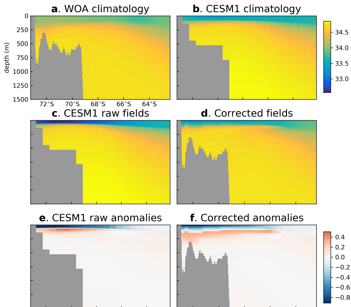
Extended Data Fig. 3 | Bias correction of salinity in physical space (depth vs latitude). The same example month as in Extended Data Fig. 2 is shown, for the eastern boundary zoomed into the depth range above 1500 m. (a) WOA climatology for July, interpolated to MITgcm grid; (b) CESM1 present-day
