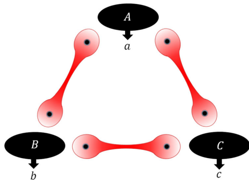
Fig. 3 Triangle network. Three nodes pairwise share pairs of entangled qubits and each perform the Elegant Joint Measurement on their respective qubit pair.
