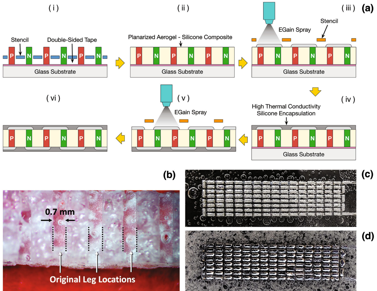
Fig. 9 Flexible TEG fabrication. a Process flow used to fabricate the flexible TEGs. b A cross-sectional microscope image of a TEG captured after physically removing the legs. c Top-view of EGaIn interconnects on a module built using pure PDMS as the filler. d Top-view of EGaIn interconnects on a module built using the aerogel-silicone composite filler.
