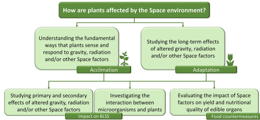
Fig. 1 Schematic view of the main knowledge gaps in plant biology which regard understanding processes of acclimation and adaptation to space factors. Understanding such processes is fundamental to evaluate the impact on the functioning of BLSS and on the value of plant-derived food for the integration of astronauts' nutrition.
