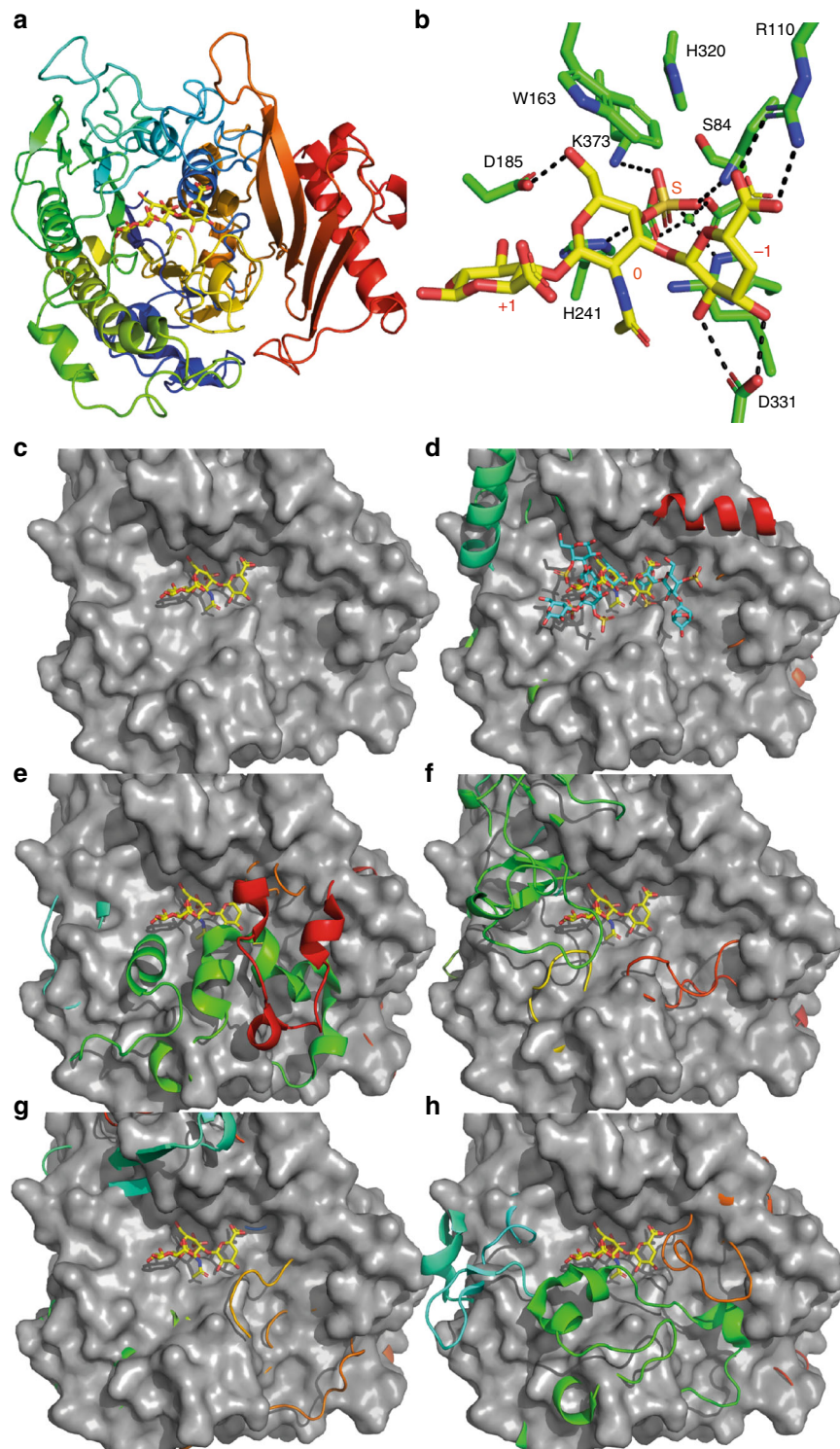
Fig. 4 Structural depictions of BT3349-S1_274 S and its comparison with other endo and exo sulfatases. a Cartoon representation of BT3349-S1_274 S -sulf ramped blue to red from its N- to C-terminus; b stick representation of binding site interactions with the protein in green and the bound trisaccharide yellow; c surface representation of BT3349-S1_274 S -sulf showing how the +1 and -1 ends of the trisaccharide are free to be extended; d overlays of surface representations of BT3349-S1_274 S -sulf and a cartoon of the marine endo 4S ι-carrageenan sulfatase (PsS1_19A). CS and ι-carrageenan oligosaccharides are shown in yellow and cyan, respectively. e Overlay of a surface of BT3349-S1_274 S -sulf with a cartoon of the exo-sulfatase BT1596-S1_92 S -sulf. f Overlay of a surface of BT3349-S1_274 S -sulf with a cartoon of the exo-sulfatase BT3333-S1_156 S -sulf. g Overlay of a surface of BT3349-S1_274 S -sulf with a cartoon of the human exo-sulfatase 1FSU 4S -sulf. h Overlay of a surface of BT3349-S1_274 S -sulf with a cartoon of the human exo-sulfatase 5FQL 2S -sulf. All cartoon representations are ramped blue to red from their N- to C-terminus.
