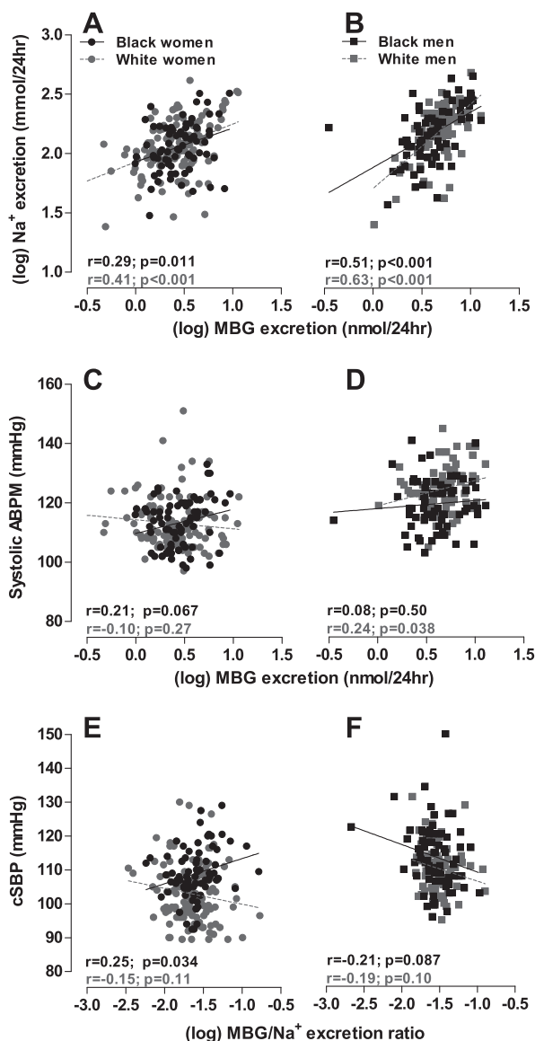
Fig. 1 Ethnic and sex differences for the relationships between \text{Na}^+ and MBG excretion (a, b); 24 h SBP and MBG excretion (c, d); and cSBP and MBG/ \text{Na}^+ excretion ratio (e, f)
