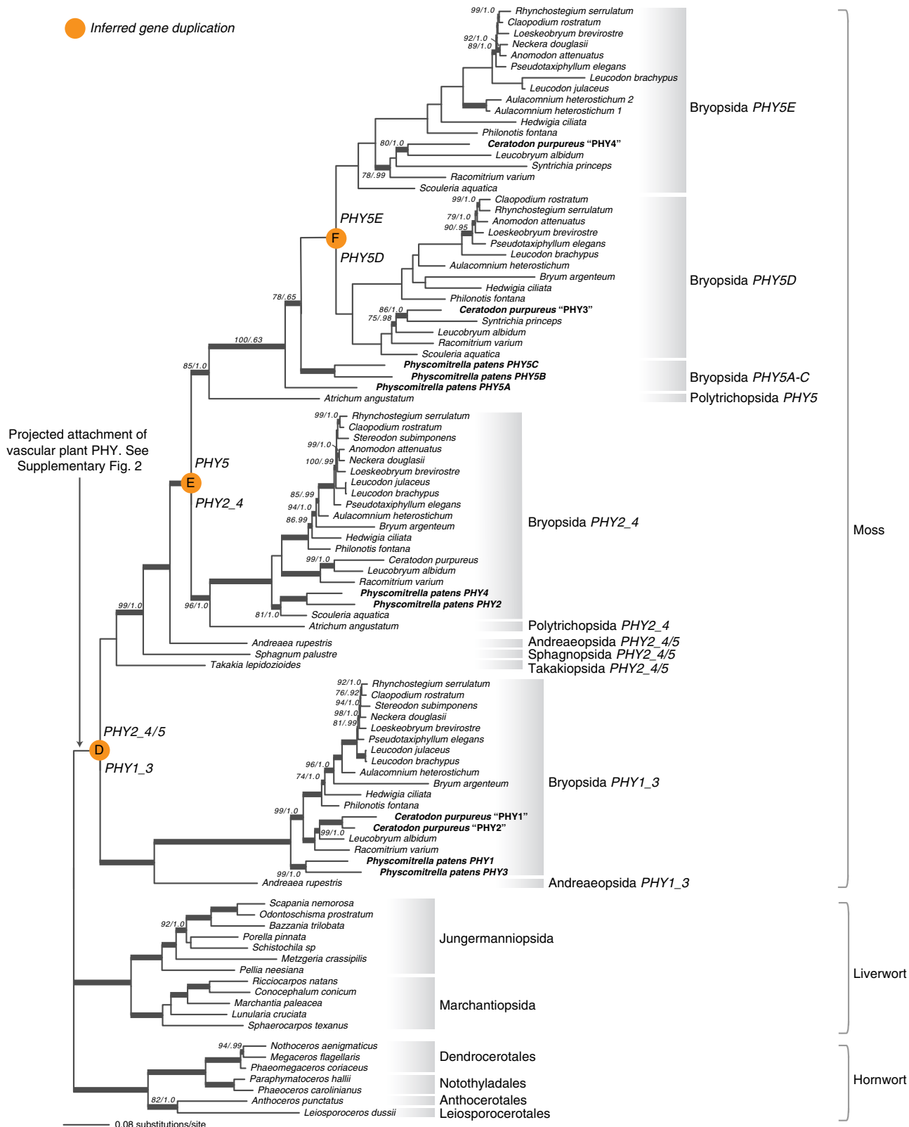
Figure 4 | Phylogeny of bryophyte phytochromes. Previously identified phytochromes are in bold font. Support values associated with branches are maximum likelihood bootstrap values (BS)/Bayesian posterior probabilities (PP); these are only displayed (along with thickened branches) if BS > 70 and PP > 0.95. Thickened branches without numbers are 100/1.0. The position of orange circles indicates inferred gene duplications. Italicized capital letters within each circle correspond to the duplication event mentioned in the text, and the numbers/letters adjacent to each circle indicate the names of the gene duplicates.
