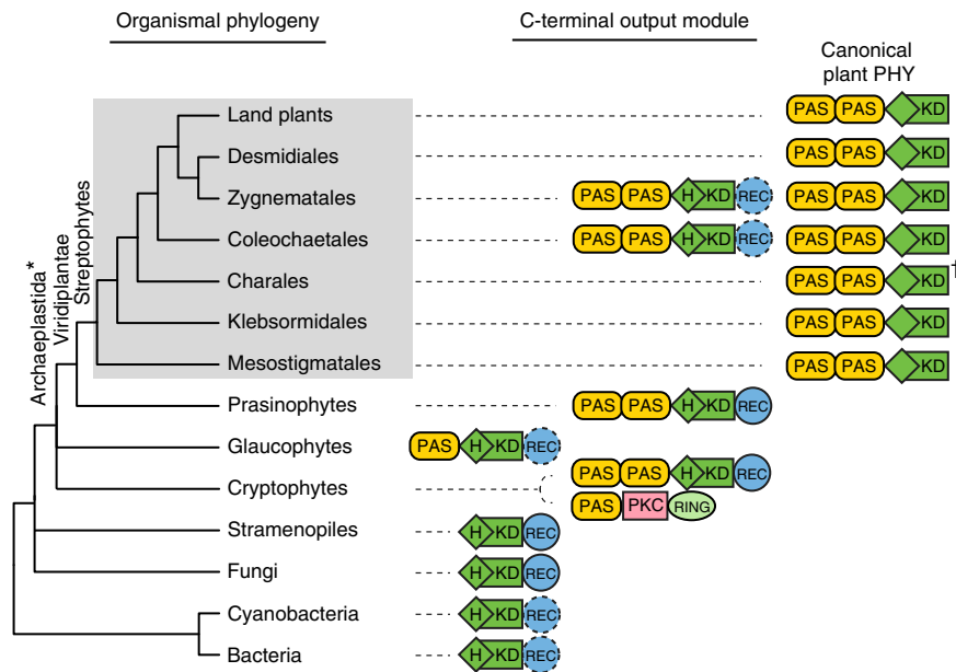
Figure 2 | The diversity and evolution of phytochrome C-terminal output module. The tree depicts the organismal phylogeny of all the phytochrome-containing lineages. The domain architecture of the C-terminal regulatory module characteristic of each lineage is indicated on the right connected by dashed lines. The N-terminal photosensory module has a largely conserved domain sequence of PAS-GAF-PHY, and is not drawn here. The substitution of the histidine phosphorylation site (H) in the histidine kinase domain (KD) occurred subsequent to the divergence of prasinophytes. The canonical plant phytochrome is restricted to streptophytes (in grey box); Zygnematales and Coleochaetales also have non-canonical plant phytochromes. Domain names: PAS (Per/Arnt/Sim); PKC (Protein Kinase C); REC (Response Regulator); and RING (Really Interesting New Gene). *Traditional Archaeplastida do not include cryptophytes 32 . †Full-length phytochrome was not available from Charales and its domain structure was inferred.
