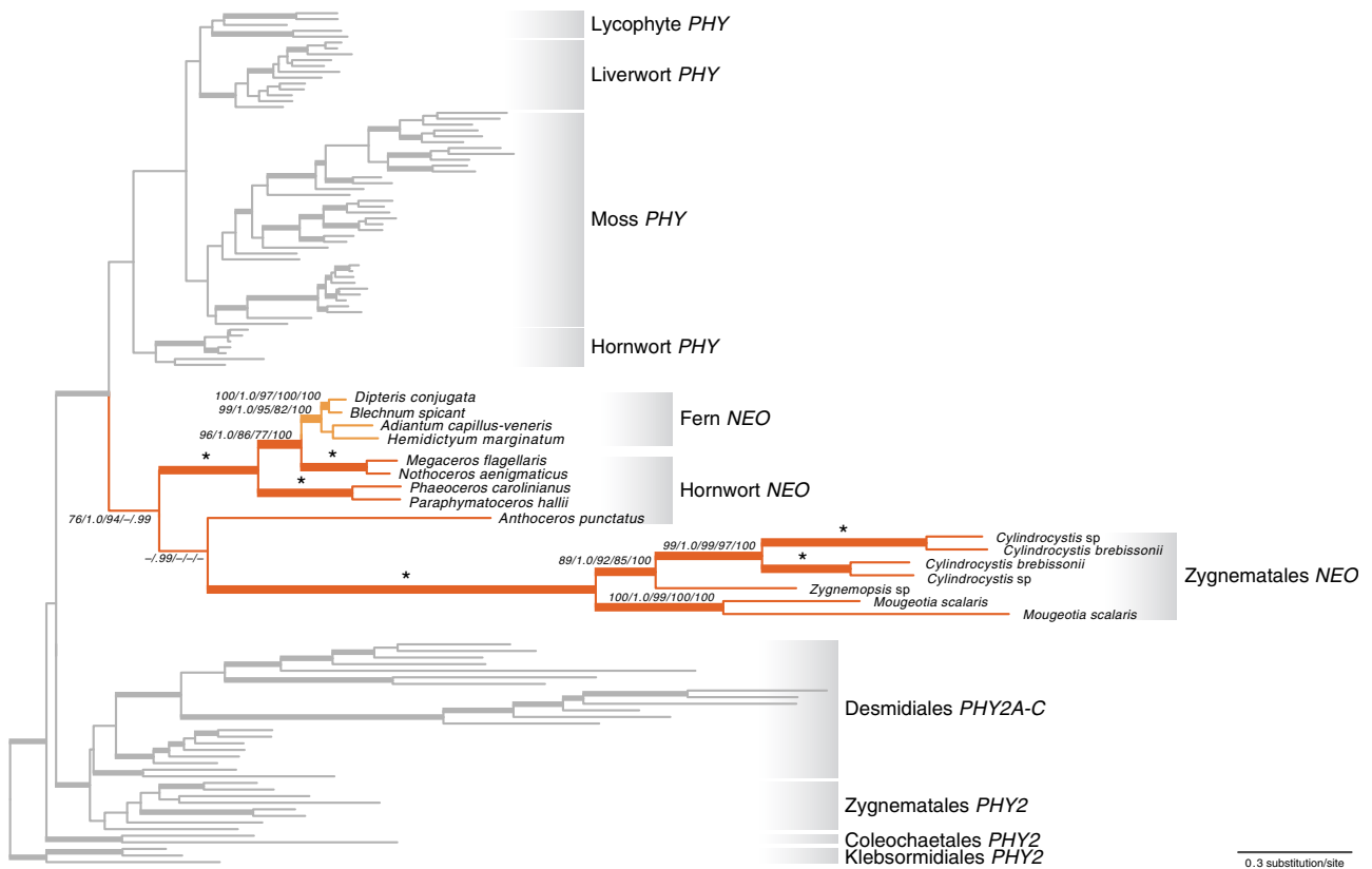
Figure 3 | Phylogeny of neochromes and phytochromes. The support values are shown for the neochrome branches only, in the following order: maximum likelihood bootstrap support (BS) from general time reversible (GTR) nucleotide model/Bayesian posterior probabilities (PP) from GTR nucleotide model/aLRT support from codon model/maximum likelihood bootstrap values from Jones-Taylor-Thornton (JTT) amino acid model/Bayesian posterior probabilities from JTT amino acid model. "*" Indicates all the support values = 100 or 1.0. "-" denotes BS < 70, aLRT < 70, or PP < 0.95. Branches are thickened when BS > 70, aLRT > 70, and PP > 0.95.
