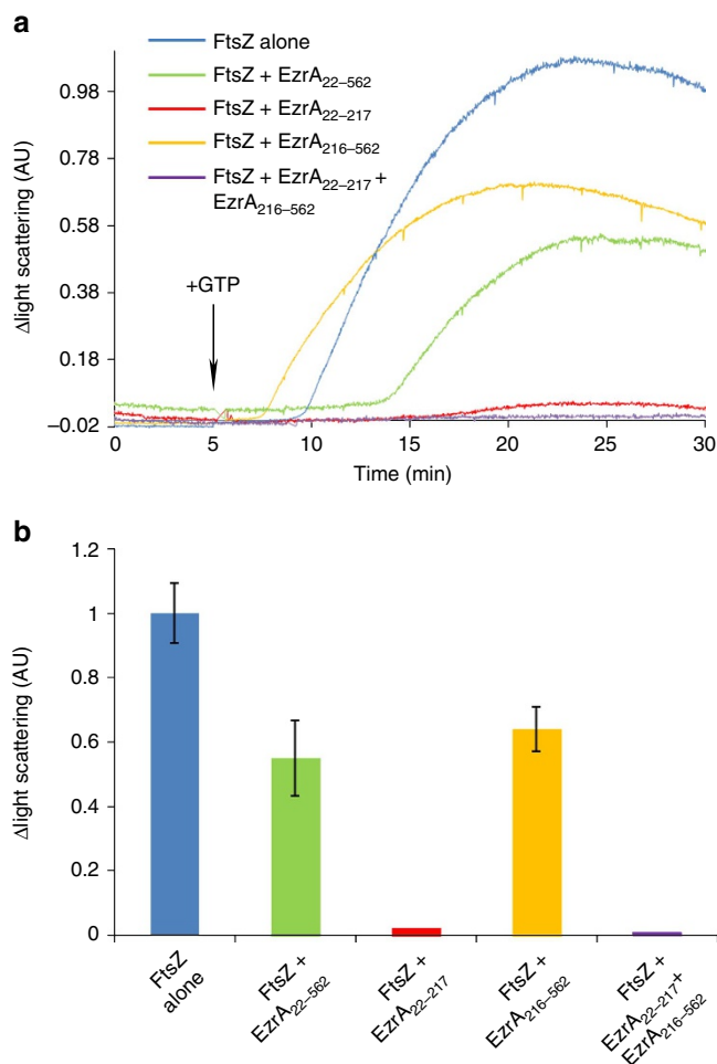
Figure 5 | Inhibition of FtsZ oligomerization by EzrA fragments.
