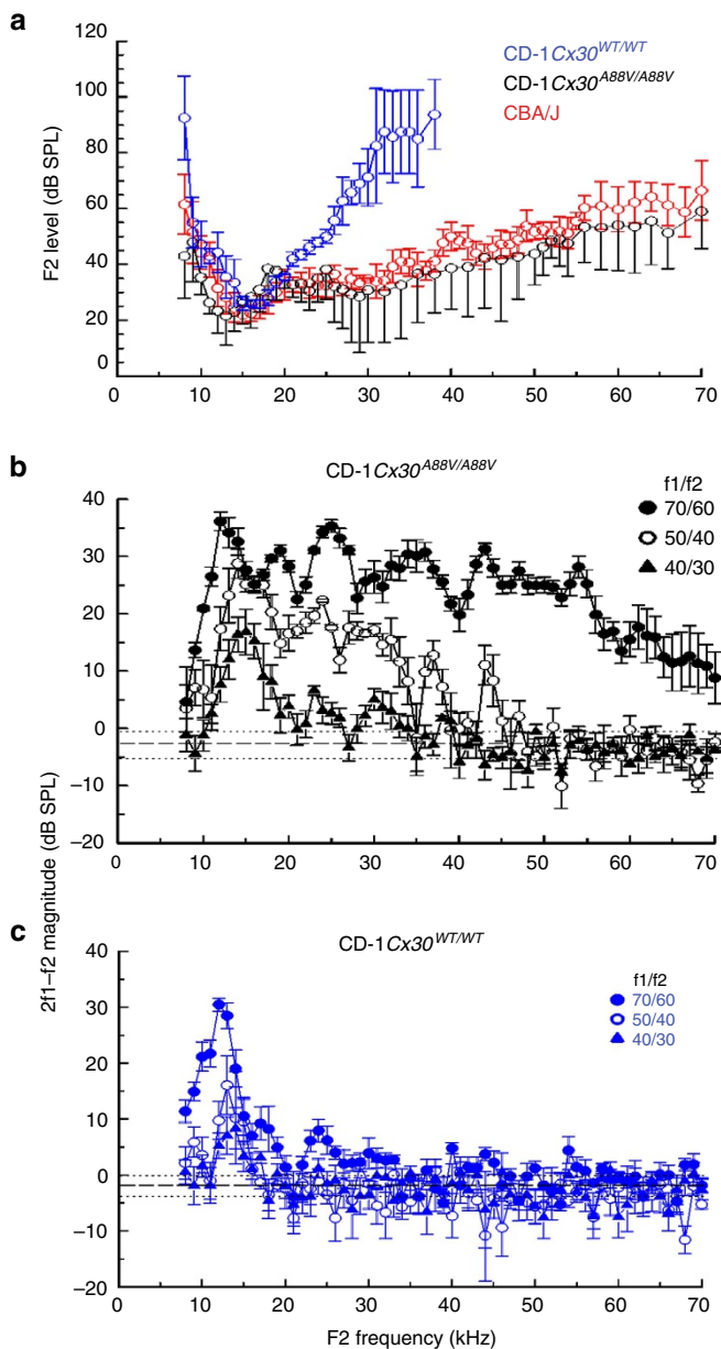
Figure 2 | DPOAE audiograms. (a) DPOAE threshold (2f 1 -f 2 , 0 dB SPL threshold criterion, mean ± s.d.) as a function of the f 2 frequency (f 2 /f 1 ratio = 1.23; level of f 2 set 10 dB below f 1 level) from six CD-1Cx30 WT/WT (blue symbols) and five CD-1Cx30 A88V/A88V (black symbols) mice, and from seven CBA/J mice (red symbols). The maximum SPL of the sound system was restricted to ≤110 dB for frequencies ≥35 kHz. (b,c) DPOAE magnitude (2f 1 -f 2 , mean ± s.d.) as a function of the f 2 frequency for five CD-1Cx30 A88V/A88V mice (b) and five CD-1Cx30 WT/WT mice (c). Stimulus levels and colour and symbol coding for f 1 and f 2 are shown in the figures. X axis: f 2 frequency (kHz). Dashed and dotted lines indicate the recording noise floor ± s.d. for all measurements.
