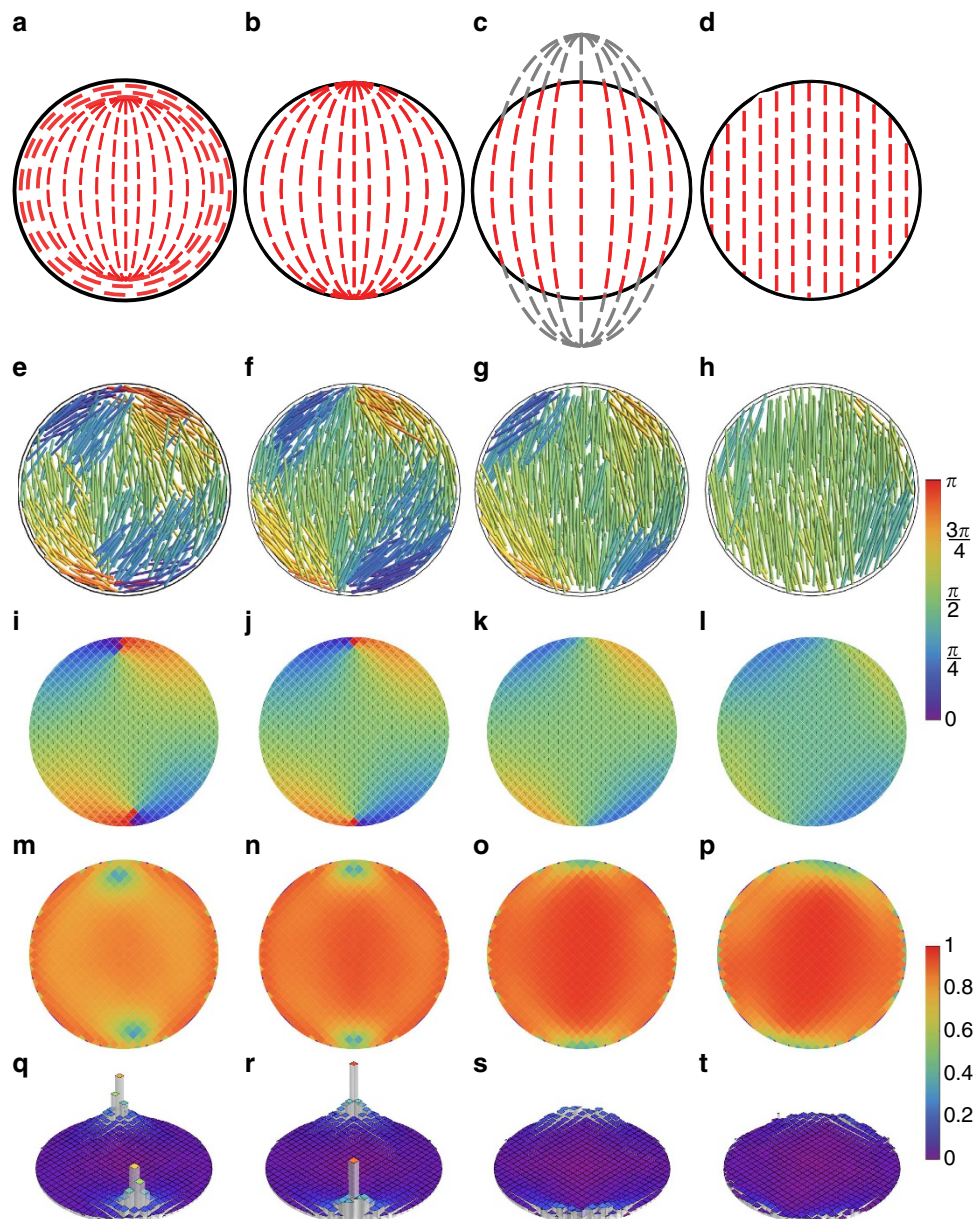
Figure 1 | Patterns of rod-like particles in circular confinement. Overview of packing structures of rod-like particles confined in shallow chambers with a circular geometry. Top row: schematic showing classification by the location of the disclination points: (a) type B_v , (b) type B_b , (c) type B_o , (d) type B_\infty . Second row: snapshots showing particle positions and their orientations with respect to the vertical ( \text{mod } \pi ) (see colour bar on the right). Third row: orientation patterns averaged over >10^3 configurations. Fourth row: value of the scalar order parameter S \in [0,1] , scale bar on the right. For a discussion of the error estimate in this quantity see the Supplementary Note 8 and Supplementary Fig. 10 Note the characteristic dips at the location of the defects. Fifth row: normalized angular deficit parameter, which peaks at the centre of the defects. Simulation parameters: (e,i,m,q) L/D = 15 and \eta = 0.16 ; (f,j,n,r) L/D = 15 and \eta = 0.20 ; (g,k,o,s) L/D = 20 and \eta = 0.20 ; (h,l,p,t) L/D = 25 and \eta = 0.20 .
