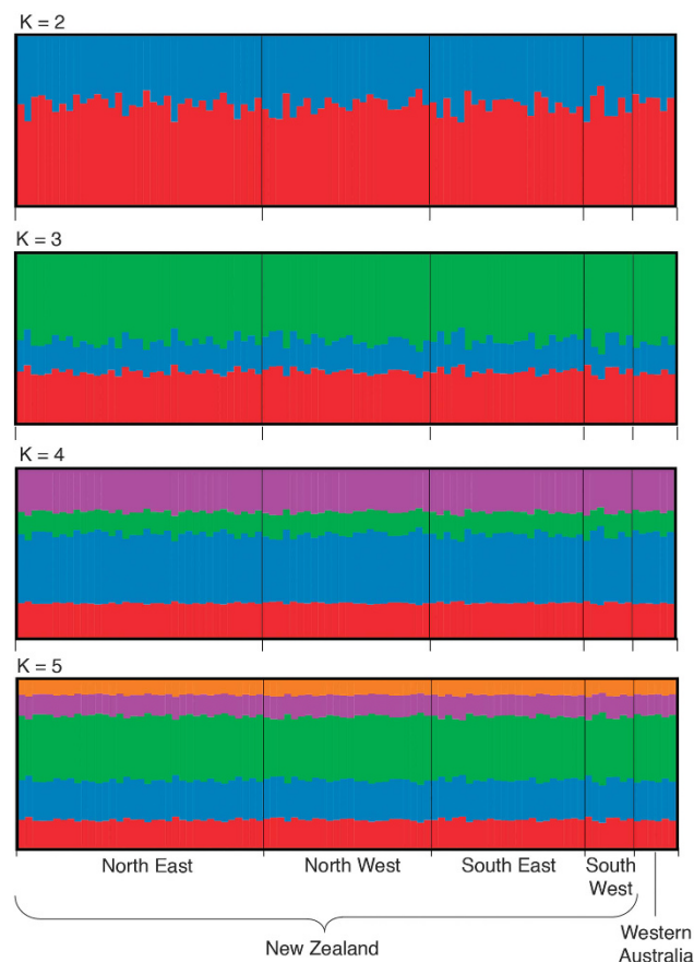
Figure 3 Bayesian STRUCTURE analysis of 12 Gray's beaked whale ( M. grayi ) microsatellite loci from five a priori regions. Each bar represents the likelihood of an individual's assignment to a particular population cluster as indicated by the colours for K = 2\text{--}5 .
