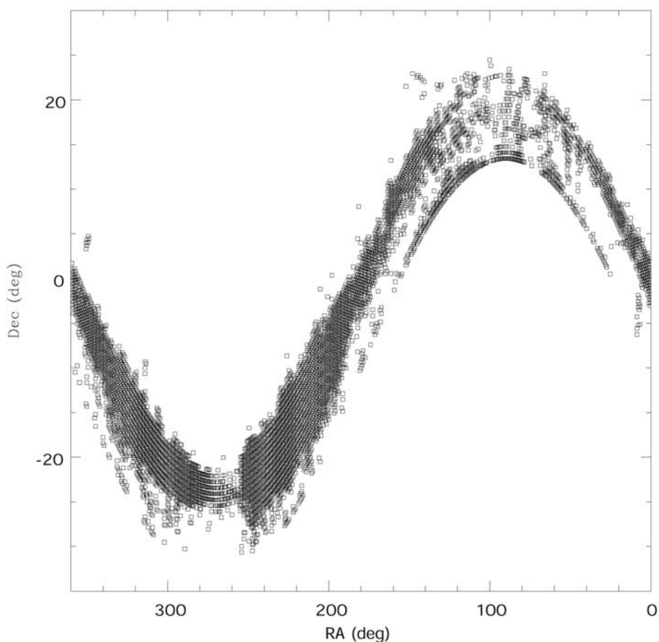
Figure 1. Plot of the fields observed by the Survey.
