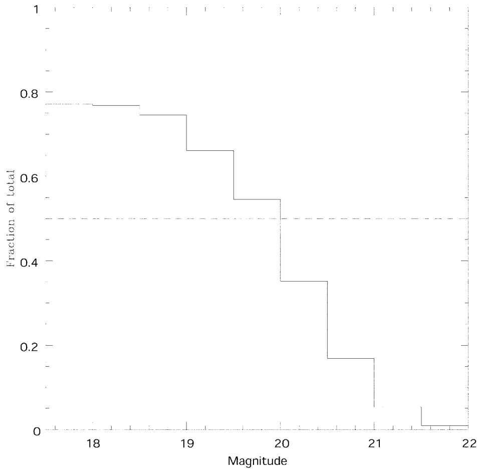
Figure 2. Detection Efficiency based on sample of 1000 fields. The dotted line indicates the 50% cutoff for the detection efficiency which for our sample is m_R \sim 19.75 .
