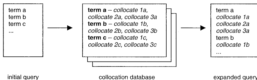
Figure 5. Query expansion with global collocates.
