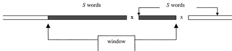
Figure 3. Right-hand half of the window truncated by hitting another occurrence of x after the node.
