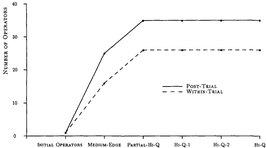
Figure 15. Growth of the operator set in within-trial and post-trial learning (Experiment 5).
