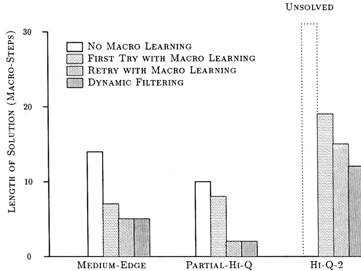
Figure 7. Lengths of solutions found with and without macro-operator learning (Experiment 1).
