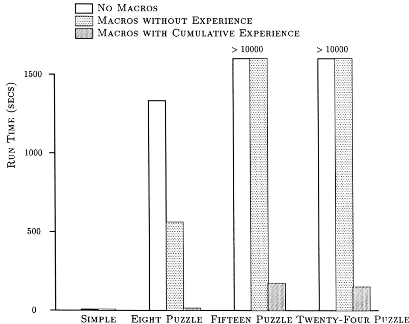
Figure 20. Run-time comparisons with and without macro learning in the tile-sliding domain using the selected-peak macro proposer (Experiment 7).
