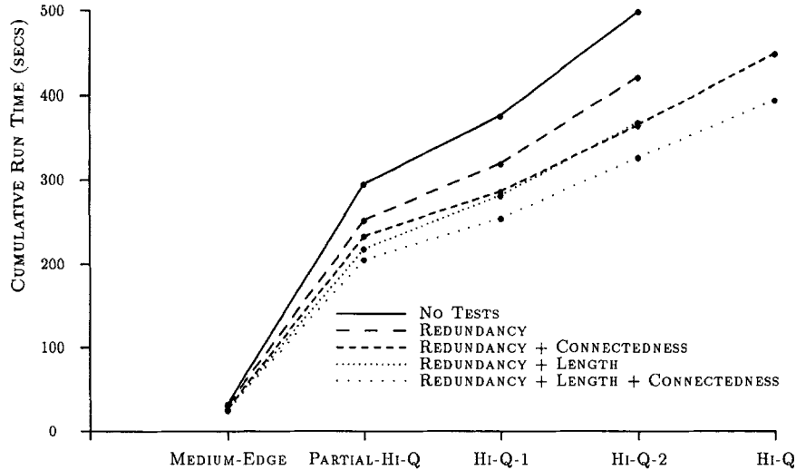
Figure 11. Cumulative run-time comparison of different static filter tests (Experiment 3).
