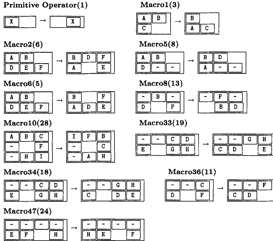
Figure 21. Full tile-sliding operator set after training on first three problems. Numbers in parentheses indicate the expanded length of each macro. Letters bind to any tile; the symbol “-” denotes a tile unchanged by a macro.
