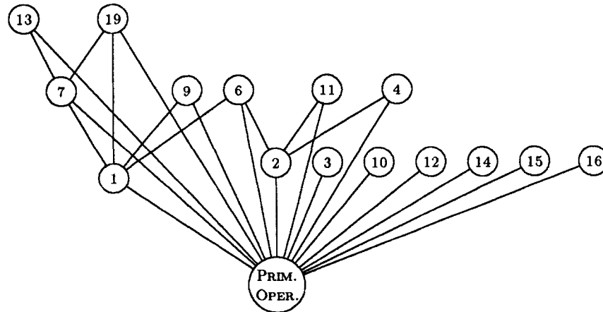
Figure 16. Hierarchy of macro definitions resulting from within-trial solving of Medium-Edge with complete static filter. Macros are represented only by their number to save space.
