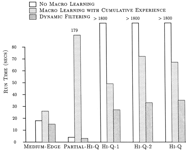
Figure 9. Run times for learning with cumulative experience (Experiment 2).
