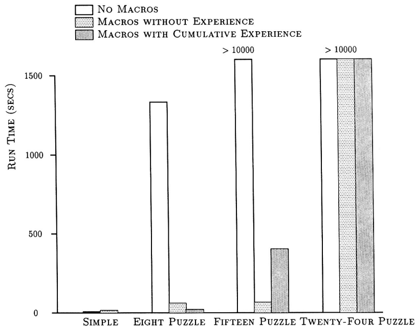
Figure 19. Run-time comparisons with and without macro learning in the tile-sliding domain using the possible-peak macro proposer (Experiment 6).
