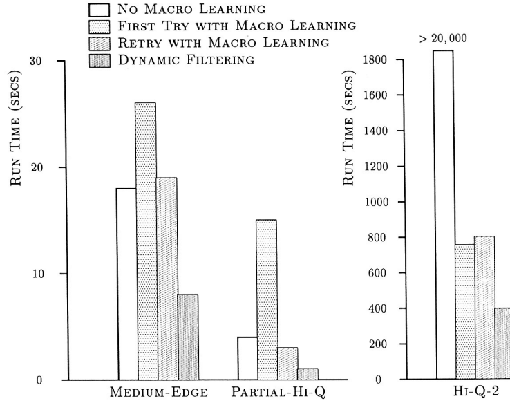
Figure 5. Run-time comparisons with and without macro learning (Experiment 1).
