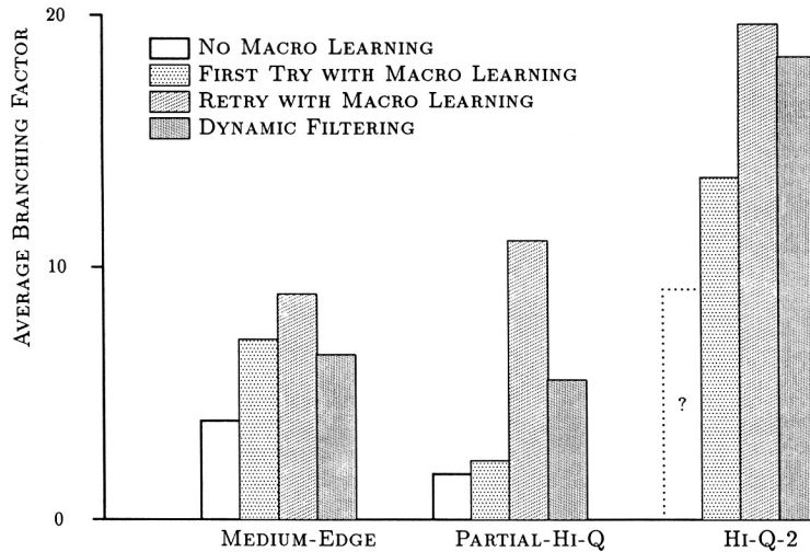
Figure 6. Average branching factors with and without macro learning (Experiment 1).
