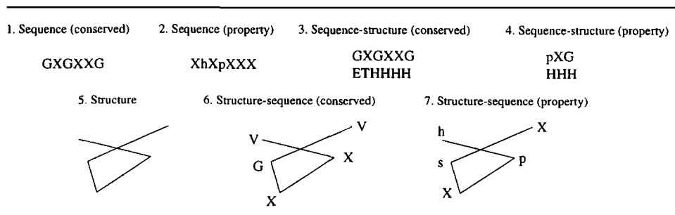
Figure 2. Various types of protein motifs. Legend; X: any residue, G: glycine, V: valine, H: helix, E: \beta -strand, T: turn, p:polar, s: small, h: hydrophobic.
