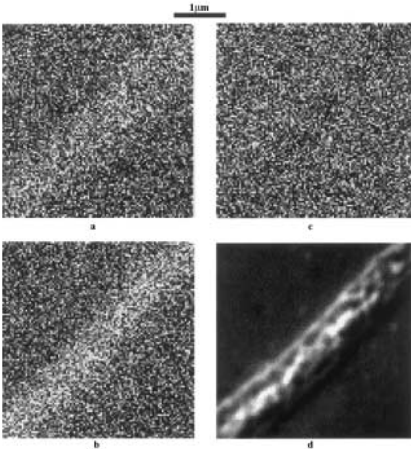
Fig. 5. Scanning Auger Spectroscopical analysis of a grain-boundary region on the surface of selectively oxidized Si-free austenitic 20Cr-25Ni stainless steel. (a) Oxygen map, (b) chromium map, (c) iron map, and (d) secondary-electron image.
