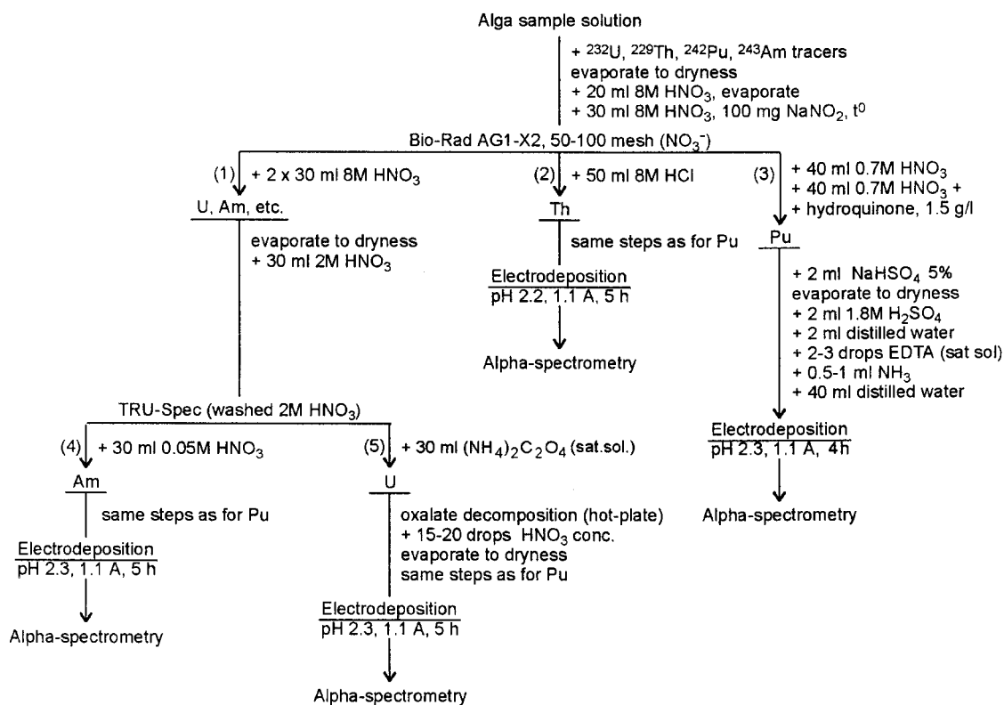
Fig. 1. Flow chart for the radiochemical analysis of U, Th, Pu and Am in alga samples
