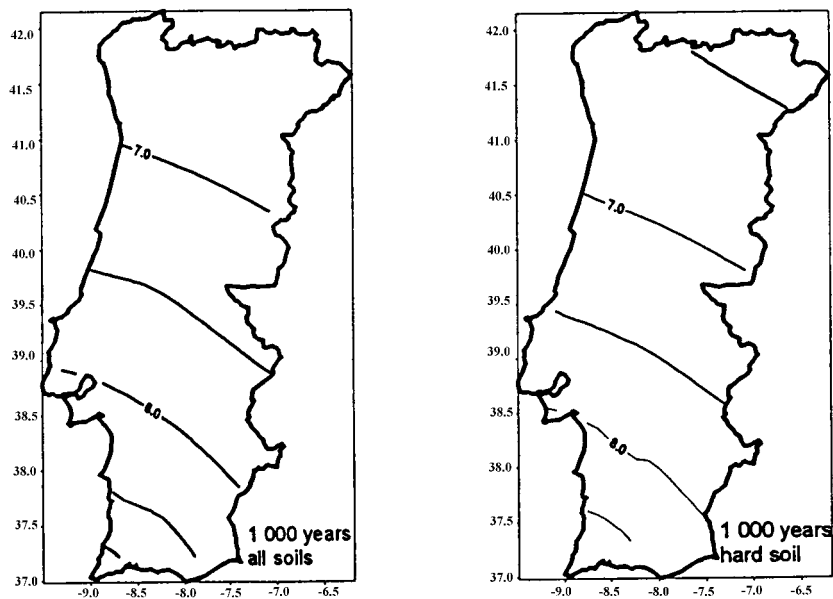
Figure 11. Seismic hazard map for 1000 years return period without soil segmentation (left) and considering only hard soil attenuation law (right).
