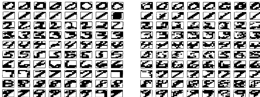
Figure 23. The leftmost figure shows examples of the images used by Saul and Jordan (1999) in training their handwritten digit classifier. The rightmost figure shows examples of images whose bottom halves were inferred from their top halves via a variational inference algorithm.
