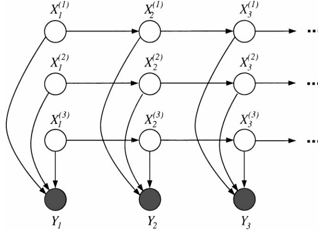
Figure 9. A factoral HMM with three chains. The transition matrices are A^{(1)} , A^{(2)} , and A^{(3)} associated with the horizontal edges, and the output probabilities are determined by matrices B^{(1)} , B^{(2)} , and B^{(3)} associated with the vertical edges.
