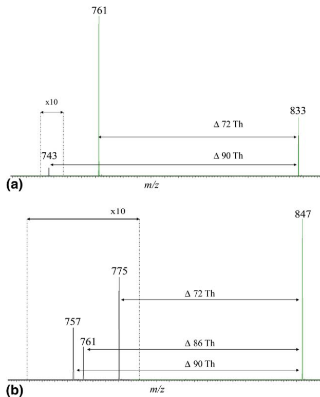
Figure 2. (a) CID spectrum of Na + cationized H-PLA-OH ( m/z 833; argon collision gas; 45 eV collision energy). (b) CID spectrum of Na + cationized CH 3 -PLA-OH ( m/z 847; argon collision gas; 45 eV collision energy).
