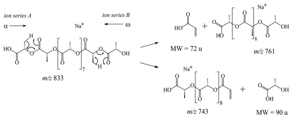
Scheme 3. Collision-induced dissociation of \text{Na}^+ -cationized H-PLA-OH oligomers: end-group specific competitive decompositions.
