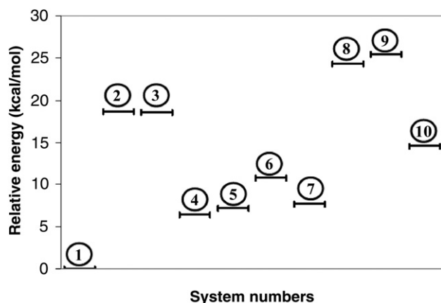
Figure 5. Relative energies of the different systems represented at Figure 4 as calculated at the DFT/B3LYP level from the most stable conformation provided by Molecular Mechanics.
