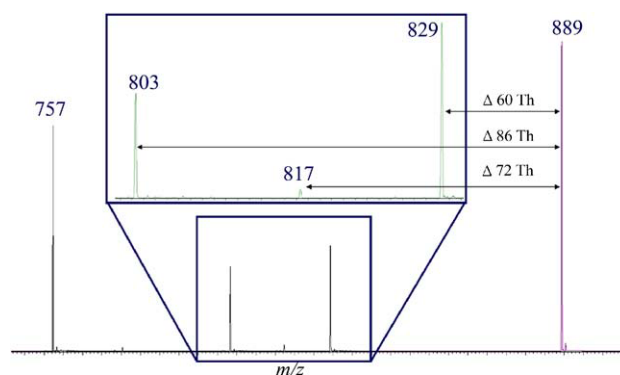
Figure 3. CID spectrum of \text{Na}^+ cationized \text{CH}_3\text{-PLA-O(C=O)CH}_3 ( m/z 889; argon collision gas; 45 eV collision energy).
