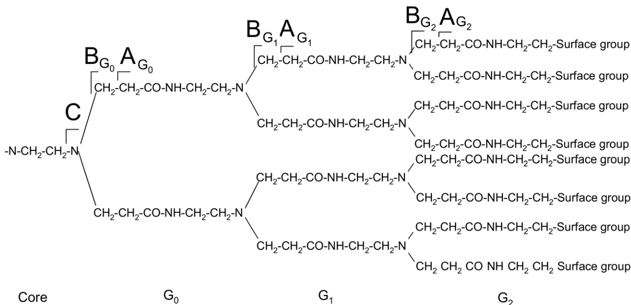
Scheme 3. Notations for representing the CID fragmentation sites along the backbone of PAMAM dendrimers (only half of the molecule is shown).
