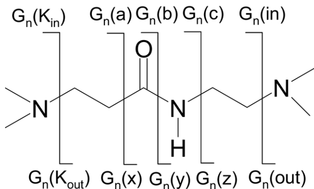
Scheme 2. Notations for representing ECD cleavage sites along the backbone of PAMAM dendrimers.
