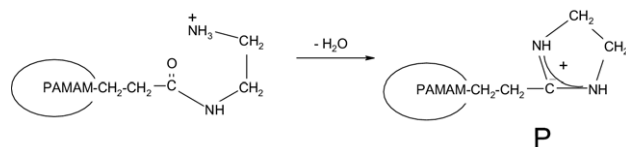
Scheme 4. Proposed mechanism for loss of water from PAMAMG1NH 2 .
