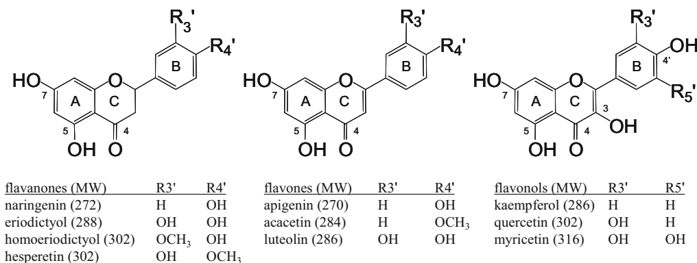
Scheme 1. Structures of flavonoid aglycons used as substrates for UGT1A1.
