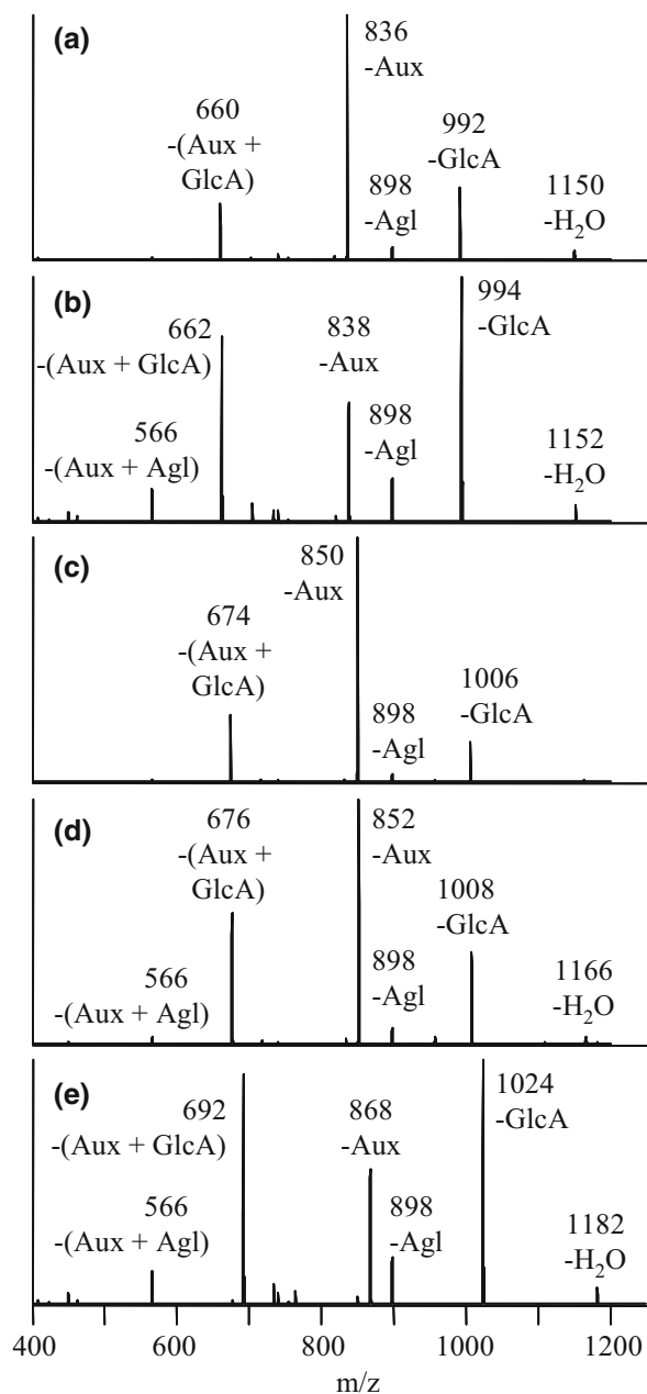
Figure 2. CID mass spectra of [\text{Co}(\text{II}) (\text{FG-H}) (4,7\text{-dpphen})_2]^+ complexes of flavonoid monoglucuronides. (a) FG = apigenin, 1168 \rightarrow (b) FG = naringenin, 1170 \rightarrow (c) FG = acacetin, 1182 \rightarrow (d) FG = kaempferol, 1184 \rightarrow (e) FG = homoeriodictyol, 1200 \rightarrow .
