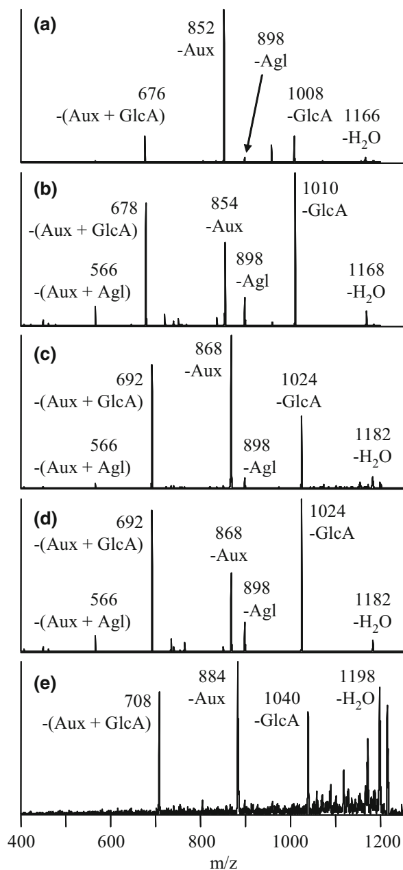
Figure 4. CID mass spectra of [\text{Co}(\text{II}) (\text{FG-H}) (4,7\text{-dpphen})_2]^+ complexes of earliest eluting flavonoid monoglucuronides from multi-product reactions. (a) FG = luteolin, 1184 \rightarrow (b) FG = eriodictyol, 1186 \rightarrow (c) FG = quercetin, 1200 \rightarrow (d) FG = hesperetin, 1200 \rightarrow (e) FG = myricetin, 1216 \rightarrow .
