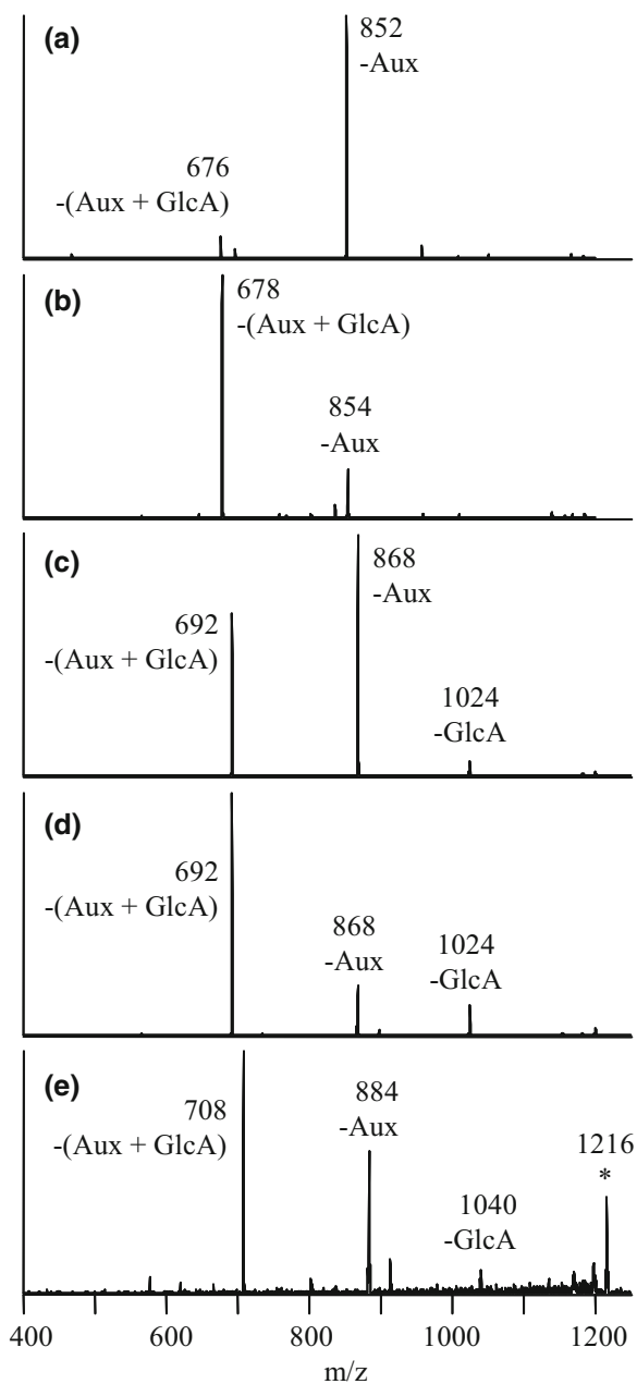
Figure 5. CID mass spectra of [\text{Co}(\text{II}) (\text{FG-H}) (4,7\text{-dpphen})_2]^+ complexes of latest eluting flavonoid monoglucuronides from multi-product reactions. (a) FG = luteolin, 1184 \rightarrow (b) FG = eriodictyol, 1186 \rightarrow (c) FG = quercetin, 1200 \rightarrow (d) FG = hesperetin, 1200 \rightarrow (e) FG = myricetin, 1216 \rightarrow .
