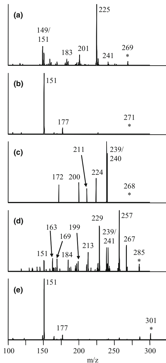
Figure 1. MS^n spectra used to confirm the identities of the aglycon skeletons of deprotonated flavonoid monoglucuronides. (a) apigenin monoglucuronide, 445 \rightarrow 269 \rightarrow (b) naringenin monoglucuronide, 447 \rightarrow 271 \rightarrow (c) acacetin monoglucuronide, 459 \rightarrow 283 \rightarrow 268 \rightarrow (d) kaempferol monoglucuronide, 461 \rightarrow 285 \rightarrow (e) homoeriodictyol monoglucuronide, 477 \rightarrow 301 \rightarrow .
