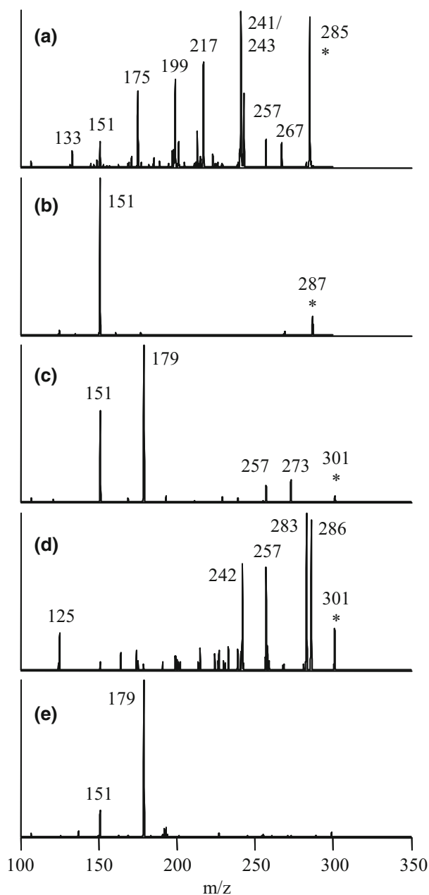
Figure 3. MS 3 spectra used to confirm the identities of the aglycon skeletons of deprotonated flavonoid monoglucuronides (earliest eluting isomer from each mixture is shown). (a) luteolin monoglucuronide, 461→285→ (b) eriodictyol monoglucuronide, 463→287→ (c) quercetin monoglucuronide, 477→301→ (d) hesperetin monoglucuronide, 477→301→ (e) myricetin monoglucuronide, 493→317→.
