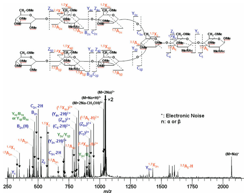
Figure 4. “Hot” ECD MS/MS spectrum of a permethylated asialo-biantennary N -linked glycan [M + 2Na]^{2+} m/z 1046.513. The cartoon structure shows observed cleavages. The peaks labeled with asterisks indicate electronic noise. The subscript x means \alpha or \beta . All the fragment ions are sodiated except the ones labeled with (H). The masses and assignments of these peaks are available in Supplemental Table S12. Glycosidic cleavages are labeled in blue, cross-ring cleavages are labeled in red, internal fragments are labeled in green.
