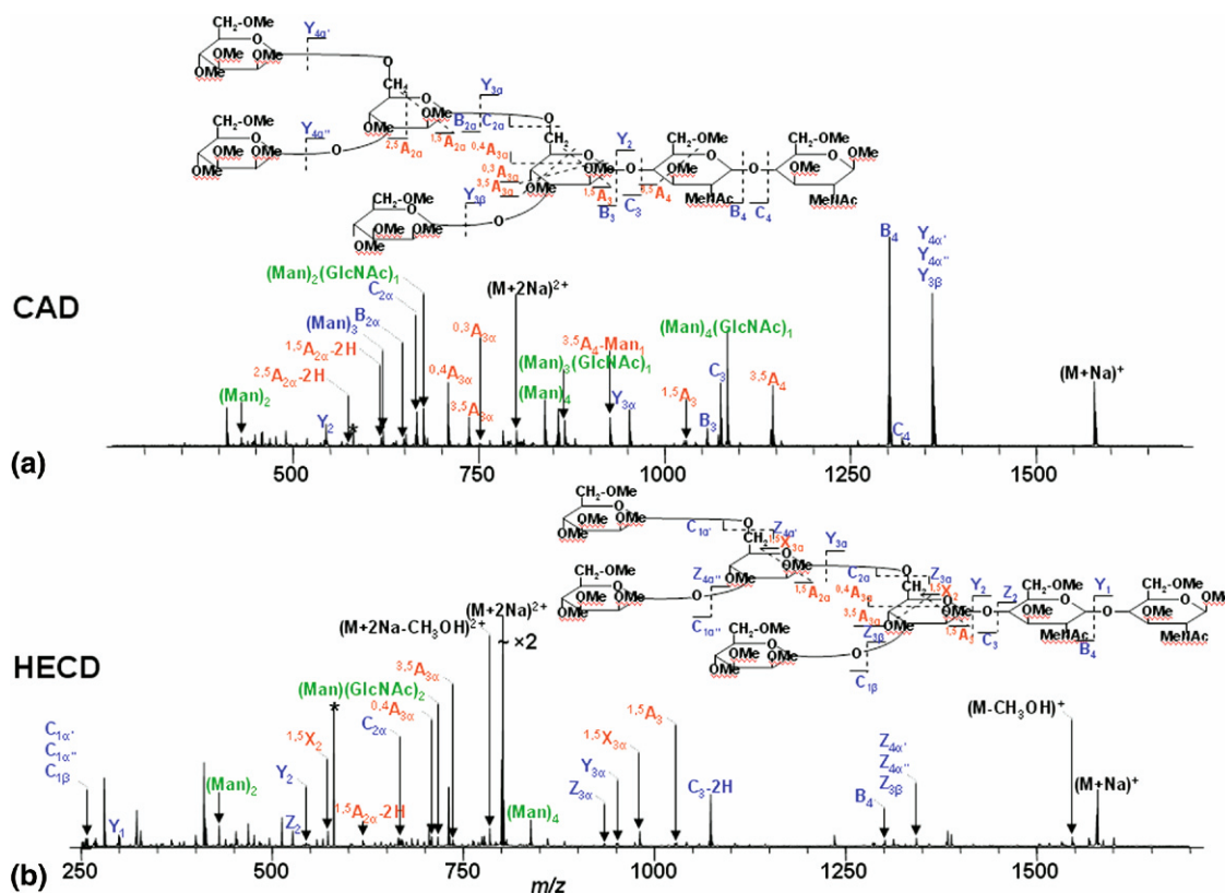
Figure 2. (a) CAD MS/MS spectrum of permethylated \text{GlcNAc}_2\text{Man}_5 [\text{M} + 2\text{Na}]^{2+} m/z 801.386. (b) “Hot” ECD MS/MS spectrum of permethylated \text{GlcNAc}_2\text{Man}_5 [\text{M} + 2\text{Na}]^{2+} m/z 801.386. All the fragment ions are sodiated except the ones labeled with (H). The peaks labeled with (2Na) are two sodiated ions. The subscript x means \alpha' or \alpha'' , or \beta . The masses and assignments of these peaks are available in Supplemental Tables S4 and S9. Glycosidic cleavages are labeled in blue, cross-ring cleavages are labeled in red, internal fragments are labeled in green.
