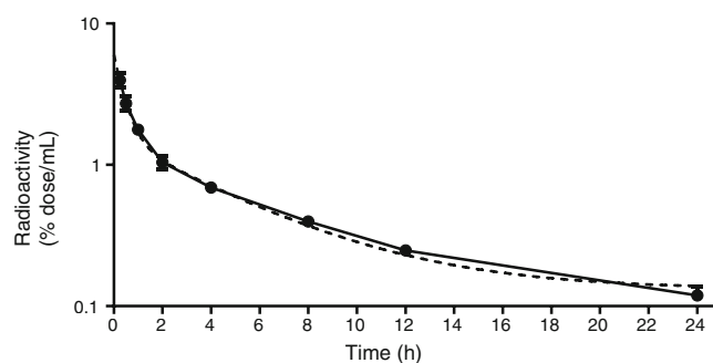
Fig. 2. Blood radioactive clearance of ^{99\text{m}}\text{Tc} -P1G10 injected in Swiss mice. Blood clearance of ^{99\text{m}}\text{Tc} -P1G10 (experimental, \bullet ) and the nonlinear theoretical regression plot (---), after i.v. administration. The ordinate is expressed as radioactivity (log scale) relative to the initial injected radioactivity (cpm) per ml of blood ( R^2 = 0.9998 ).
