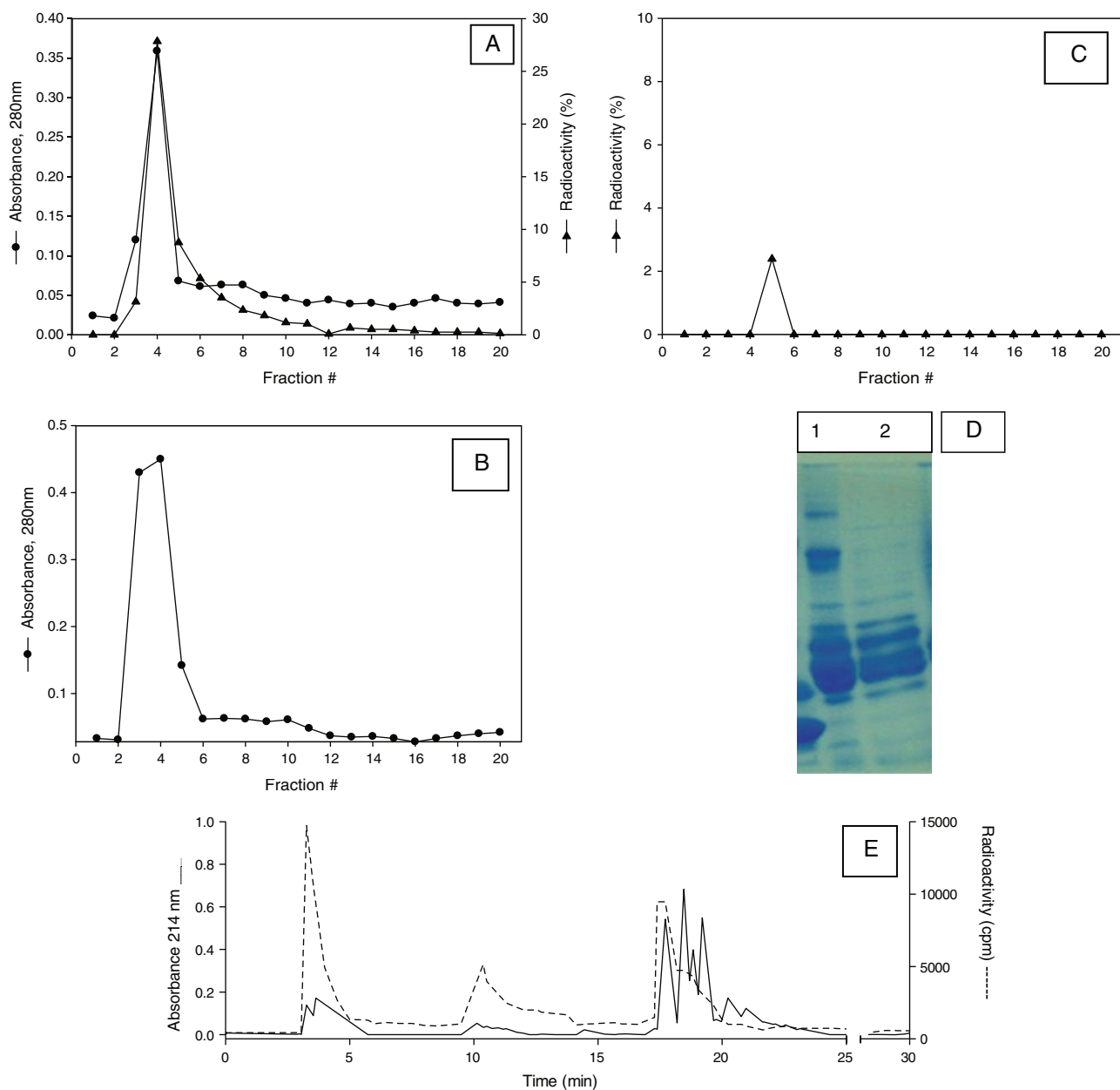
Fig. 1. Chromatographic purification and characterization of radiolabeled ^{99m}\text{Tc} PIG10. (A) ^{99m}\text{Tc} -PIG10, (B) PIG10 and (C) ^{99m}\text{TcO}_4^- + ^{99m}\text{TcO}_2 after filtration in Sephadex G-15 column. Two hundred microliters of PIG10 (5 \mu\text{g}/\mu\text{l} ) or ^{99m}\text{Tc} -PIG10 (5 \mu\text{g}/\mu\text{l} – 1 mCi), or ^{99m}\text{TcO}_4^- + ^{99m}\text{TcO}_2 (3.7 MBq) were applied onto Sephadex G-15 column. Fractions (0.7 ml) were collected at flow rate 0.7 ml/min. The protein profile was determined at 280 nm and the radioactivity assessed in a dose calibrator Capintec. (D) SDS-PAGE electrophoresis of PIG10 and ^{99m}\text{Tc} -PIG10. Heat-denatured protein samples (30 \mu\text{g} ) were loaded onto each lane. Lane 1; PIG10. Lane 2 ^{99m}\text{Tc} -PIG10. (E) HPLC reverse-phase chromatography of ^{99m}\text{Tc} -PIG10. The C4 column (Vydac) was equilibrated with 0% acetonitrile – 0.1% TFA before injection of PIG10 dissolved in milli-Q water followed by elution with a non-linear acetonitrile – 0.1% TFA gradient at a flow rate of 1 ml/min (0–54% acetonitrile for 20 min; 54–81% acetonitrile for 10 min; 81–90% acetonitrile for 10 min).
