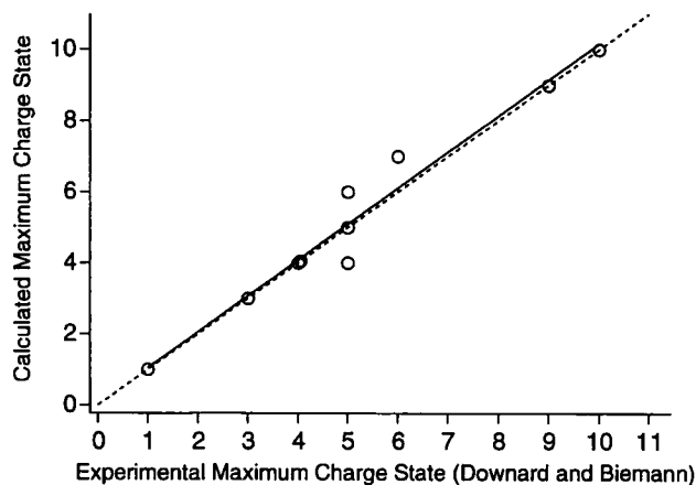
Figure 4. Calculated maximum charge state with flexible terminus modification ( \circ ). The solid line is obtained from a linear best fit and the dashed line indicates an ideal fit. Overlapping points are offset.
