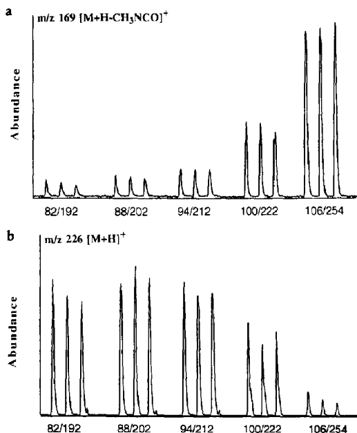
Figure 5. (a) Ion intensities of the fragment ions [M + H - CH_3NCO]^+ , m/z 169, and (b) the quasimolecular ion, m/z 226, in PI-TSP mass spectra of 5- \mu g methiocarb as a function of the nebulizer temperature (stem temperature-probe tip temperatures). 50:50 methanol-water was used as the carrier stream.
