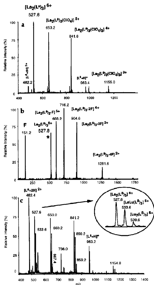
Figure 6. IS-MS spectra of the triple helical [\text{La}_2(\text{L}^8)_3(\text{ClO}_4)_6] complex from pure acetonitrile solutions. (a) Single scan mass spectrum \Delta V = 10 V; (b) product ion mass spectrum of [\text{La}_2(\text{L}^8)_3]^{6+} m/z 527.8 (CGT = 369 \times 10^{12} atoms/cm 2 ; E = 330 eV); (c) single scan spectrum of the heterodinuclear complex [\text{LaLu}(\text{L}^8)_3(\text{ClO}_4)_6] , \Delta V = 0 V.
