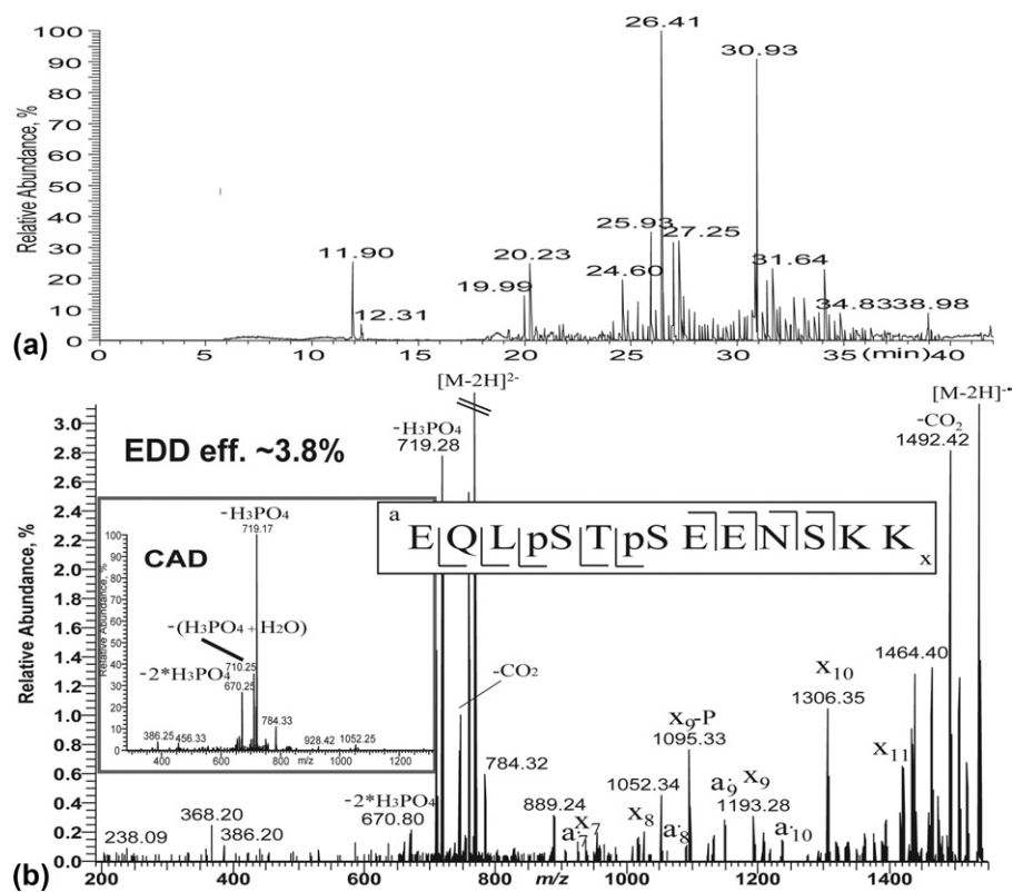
Figure 4. (a) Total ion chromatogram and (b) EDD mass spectrum of the doubly phosphorylated peptide EQLpSTpSEENSKK ( m/z 768.3, z = 2 ). All EDD-MS/MS spectra consist of four summed acquisitions.
