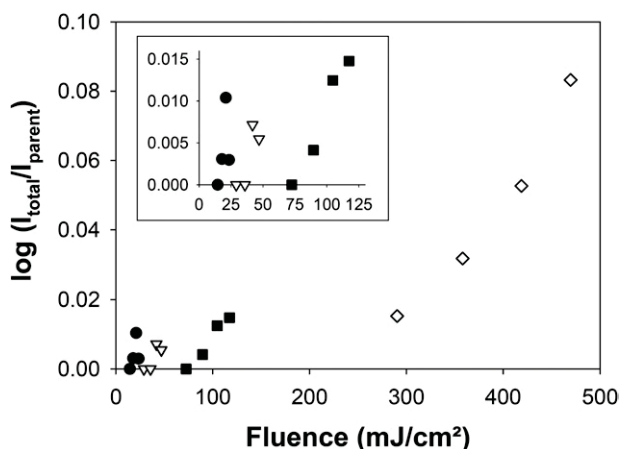
Figure 5. Relative photodetachment yield of [dsB + Ethidium] 5- at 500 nm as a function of the total laser fluence (fluence per laser pulse multiplied by the number of pulses). ● = 1 laser pulse, ▽ = 2 laser pulses, ■ = 5 laser pulses, and ◇ = 20 laser pulses. The inset shows a zoom on the low fluence region.
