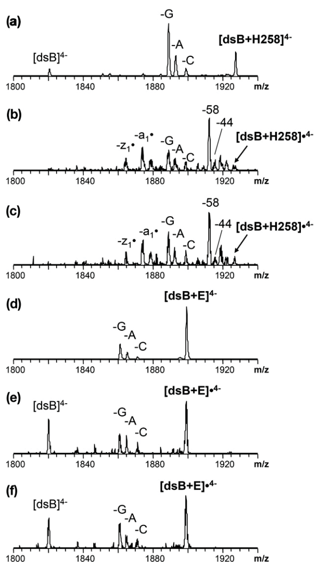
Figure 4. Comparison of CID of closed shell and radical ions from the ligand-DNA complexes. (a) CID during 30 ms at 10% activation amplitude on [\text{dsB} + \text{Hoechst 33258}]^{4-} produced by electrospray. (b) CID during 30 ms at 10% activation amplitude on [\text{dsB} + \text{Hoechst 33258}]^{4-} produced by electron photodetachment of [\text{dsB} + \text{Hoechst 33258}]^{5-} under 2-s irradiation at 260 nm. (c) CID during 30 ms at 10% activation amplitude on [\text{dsB} + \text{Hoechst 33258}]^{4-} produced by electron photodetachment of [\text{dsB} + \text{Hoechst 33258}]^{5-} under 5-s irradiation at 355 nm. (d) CID during 30 ms at 9% activation amplitude on [\text{dsB} + \text{Ethidium}]^{4-} produced by electrospray. (e) CID during 30 ms at 9% activation amplitude on [\text{dsB} + \text{Ethidium}]^{4-} produced by electron photodetachment of [\text{dsB} + \text{Ethidium}]^{5-} under 2-s irradiation at 260 nm. (f) CID during 30 ms at 9% activation amplitude on [\text{dsB} + \text{Ethidium}]^{4-} produced by electron photodetachment of [\text{dsB} + \text{Ethidium}]^{5-} under 2-s irradiation at 550 nm.
