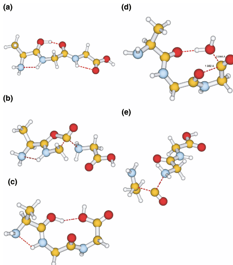
Figure 1. Selected structures on the potential energy surface of protonated AGG: (a) global minimum, (b) TS b 2 -y 1 on the b 2 -y 1 PFP, (c) RC H 2 O_loss and (d) TS H 2 O_loss on the water loss PFP, and (e) TS a 1 -y 2 on the a 1 -y 2 PFP.
