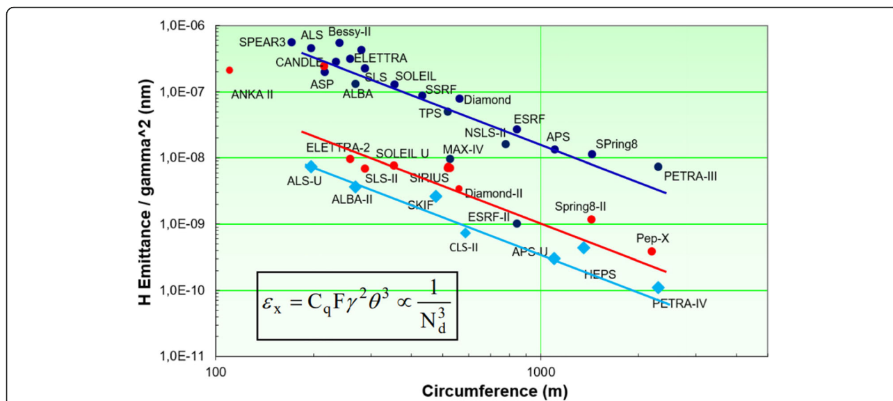
Fig. 9 Storage ring distributions along circumference [25]
