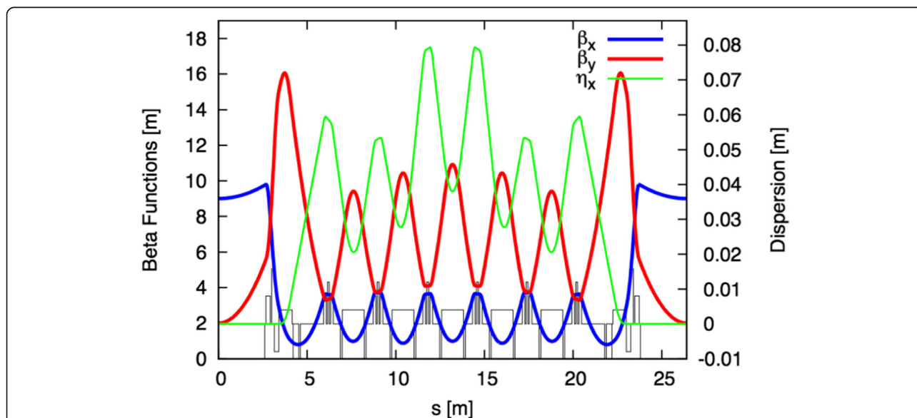
Fig. 10 Classical multi-bend achromat lattice [19]
