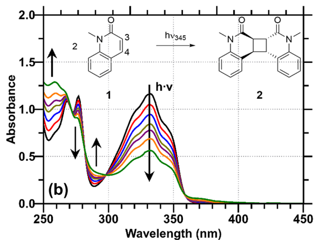
Fig. 1 a Absorption spectra of NMQ (1) and NMQ-dimer (2). The concentration of both compounds was 0.015 mM. The LED light source emits the spectrum shown which is centered at 345 nm. b UV/Vis difference spectra tracing the [2 + 2]-cycloaddition of NMQ (1)
