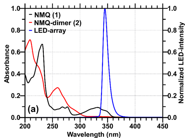
Fig. 1 a Absorption spectra of NMQ (1) and NMQ-dimer (2). The concentration of both compounds was 0.015 mM. The LED light source emits the spectrum shown which is centered at 345 nm. b UV/Vis difference spectra tracing the [2 + 2]-cycloaddition of NMQ (1)
