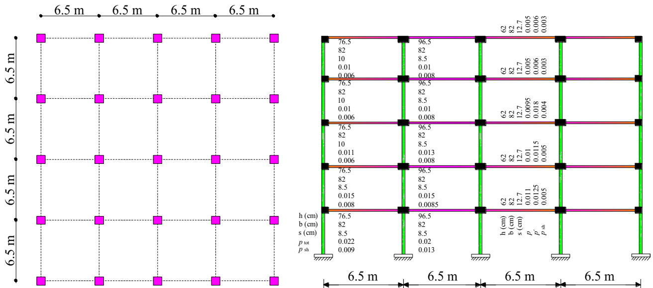
Fig. 15 A five-Story RC frame is used for the performance evaluation of trained prediction models
