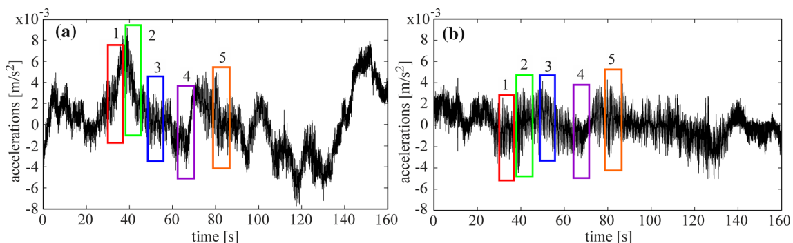
Fig. 4 Response of horizontal acceleration of the tower with selected signal intervals (1–5) for ERA calculations: a sensor A4, b sensor A5
