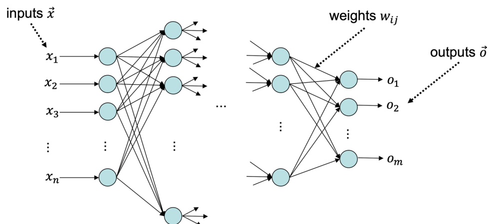
Fig. 2 Schematic illustration of a feed-forward neural network: Neurons are shown in light blue. The input layer is shown on the left, the output layer on the right. In between, there can be several hidden layers with an arbitrary number of neurons
