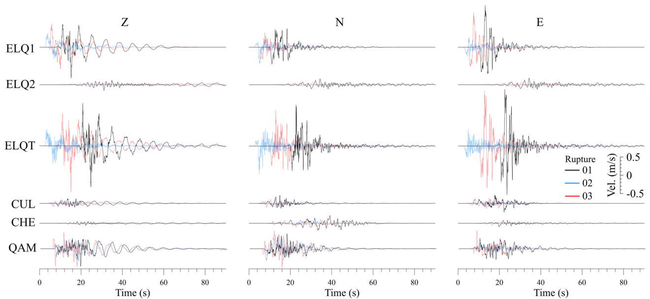
Fig. 15 Summary of velocity proportional ground motions at the CAB for all six sources which are labeled at the left of the seismograms. The left middle and right columns show the vertical ( Z ), north-south ( N ), and east-west ( E ) components of the ground
