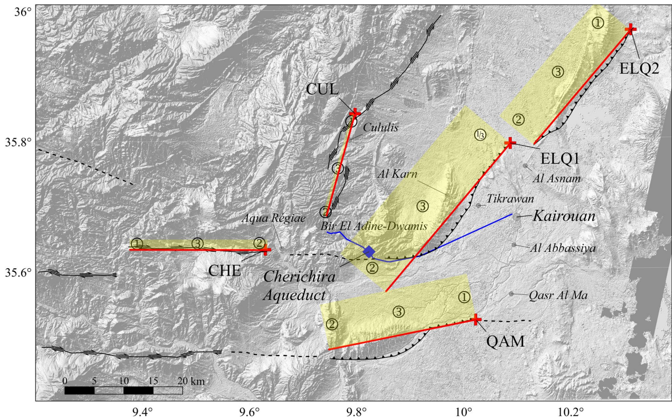
Fig. 14 Source model for the Kairouan area. Black lines show the major fault elements. Red lines are the surface traces of the rectangular fault segments. The red crosses show the reference points for the sources (Table 5) and the yellow shaded areas indicate the surface projection of the idealized fault planes. Black circles numbered 1, 2, and 3 indicate the epicenters for three rupture processes for each
