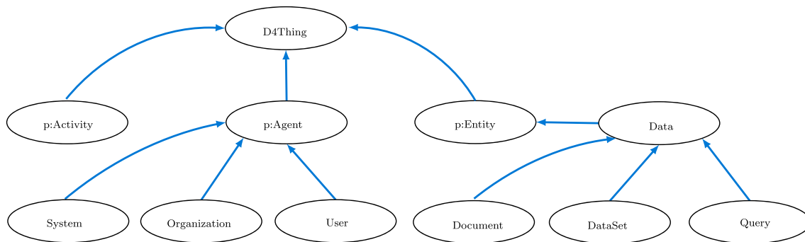
Fig. 2 Abstract shared model, with arrows denoting the type-of relation
