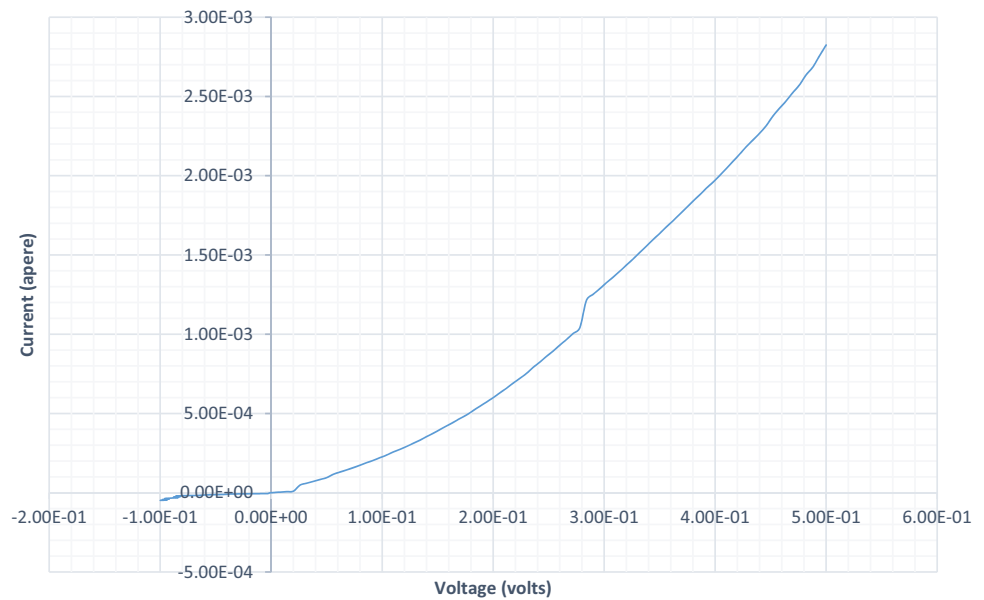
Fig. 10 Current–voltage characteristics for ZnO.NPs thin film device
