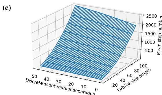
Fig. 4 a Results plotted for simulation 1 for n = 50 with fit found via method of least squares, following Eq. (26), with the corresponding constants found in Table 1. All other figures for lattice size \{10, 20, \dots, 100\} \setminus \{50\} are in Fig. 7. b–c Visualizations of all fitted plots from all lattice sizes. b shows all the fitted plots on the same axis as the plots for all lattice sizes, while c displays the surface found by plotting the fitted plots against the lattice size
