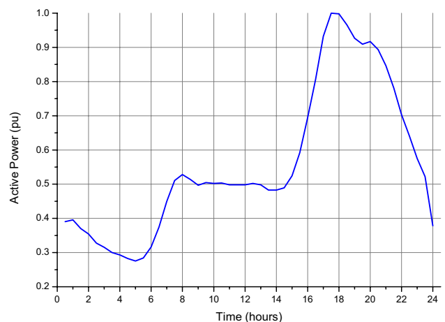
Fig. 6 Typical residential load profiles (day of maximum demand) [15]
