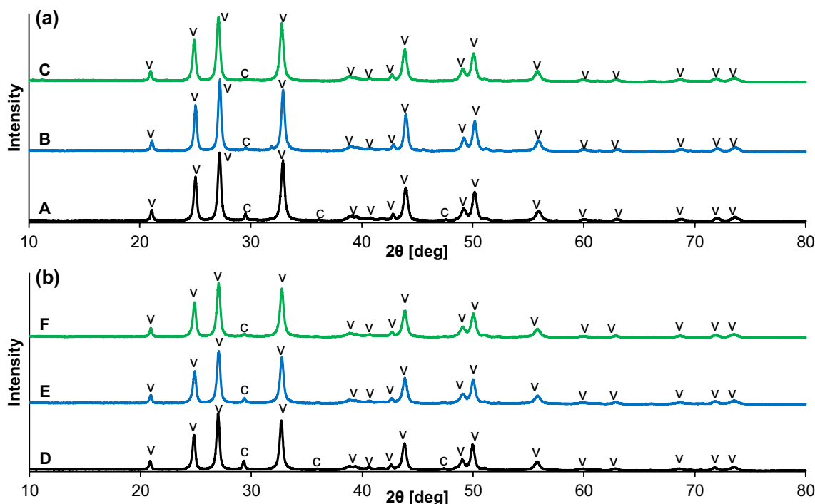
Fig. 4 XRD patterns of obtained CaCO 3 particles produced using a pure CO 2 (a) and a mixture CO 2 —air X_{V,CO_2} = 0.15 (b) depending on the ammonia concentration (c calcite, v vaterite)
