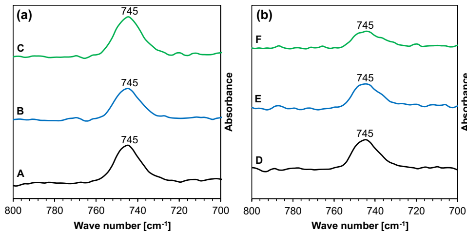
Fig. 3 FT-IR spectra of obtained CaCO 3 particles produced using a pure CO 2 (a) and a mixture CO 2 —air X_{V,CO_2} = 0.15 (b) depending on the ammonia concentration
