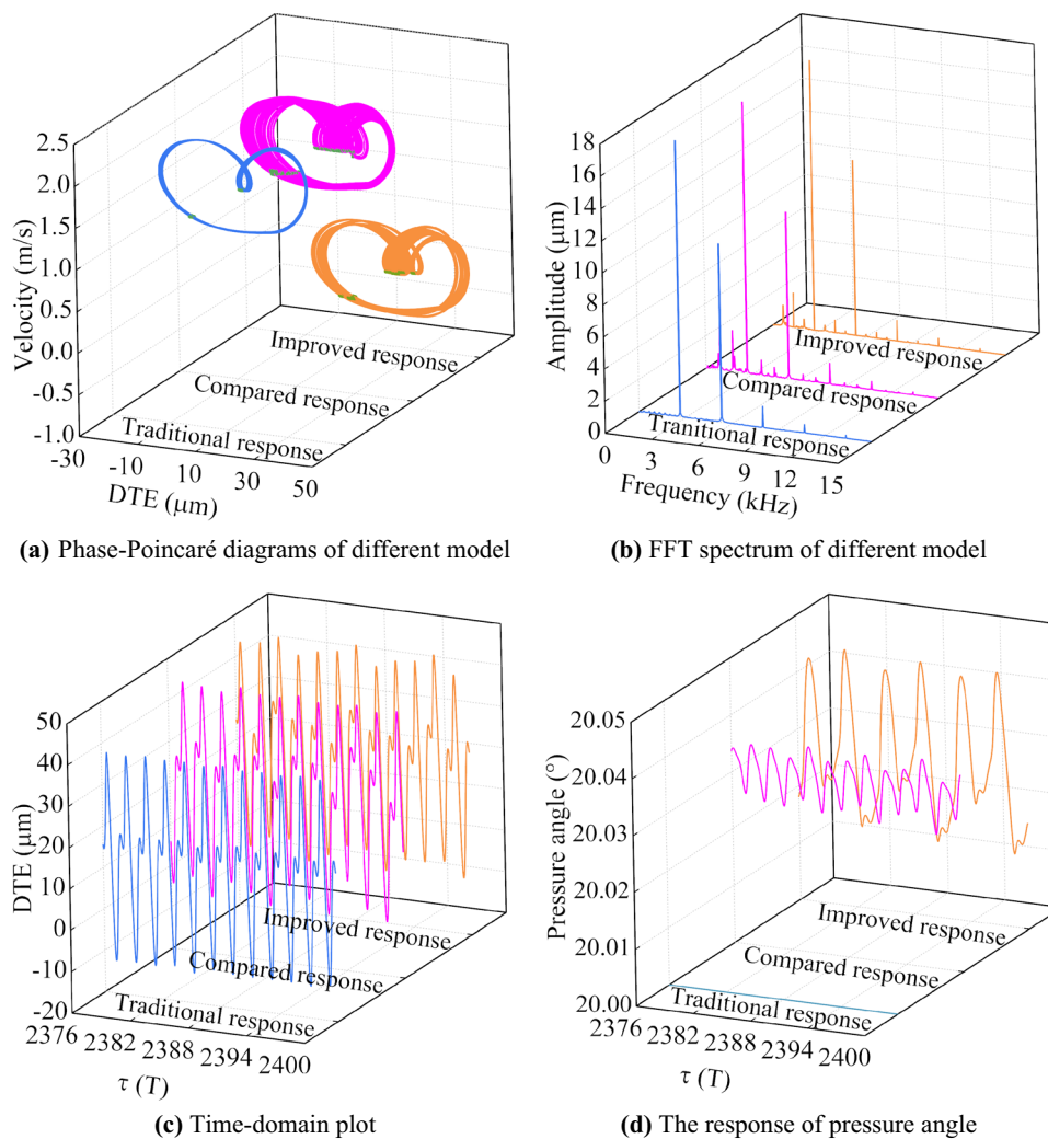
Fig. 5 Dynamic feature with fractal backlash around n = 8000 r/min
