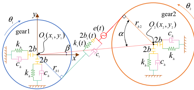
Fig. 1 Dynamic model of the gear-bearing system
