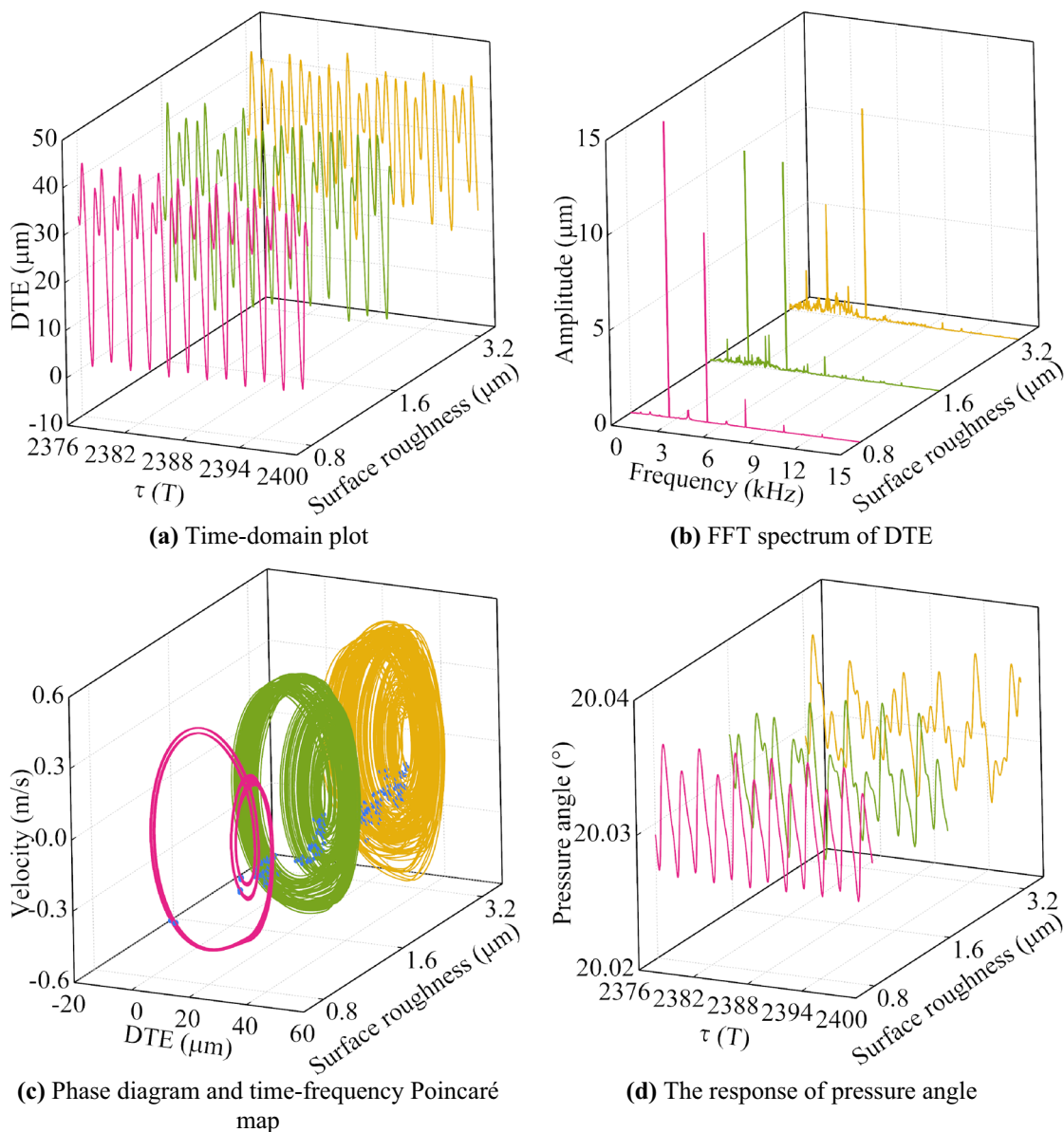
Fig. 7 Dynamic characteristic by different surface roughness
