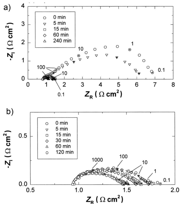
Fig. 13 Impedance plots of a \text{La}_{0.72}\text{Sr}_{0.18}\text{MnO}_3 electrode a before and b after acid treatment with 1 M HCl solution for ORR as a function of cathodic polarization at 200 \text{ mA cm}^{-2} and 900^\circ\text{C} in air. Impedance was measured under an open circuit and frequency numbers are shown in Hz. Reproduced with permission from Ref. [53]. Copyright 2001, Elsevier Inc.
