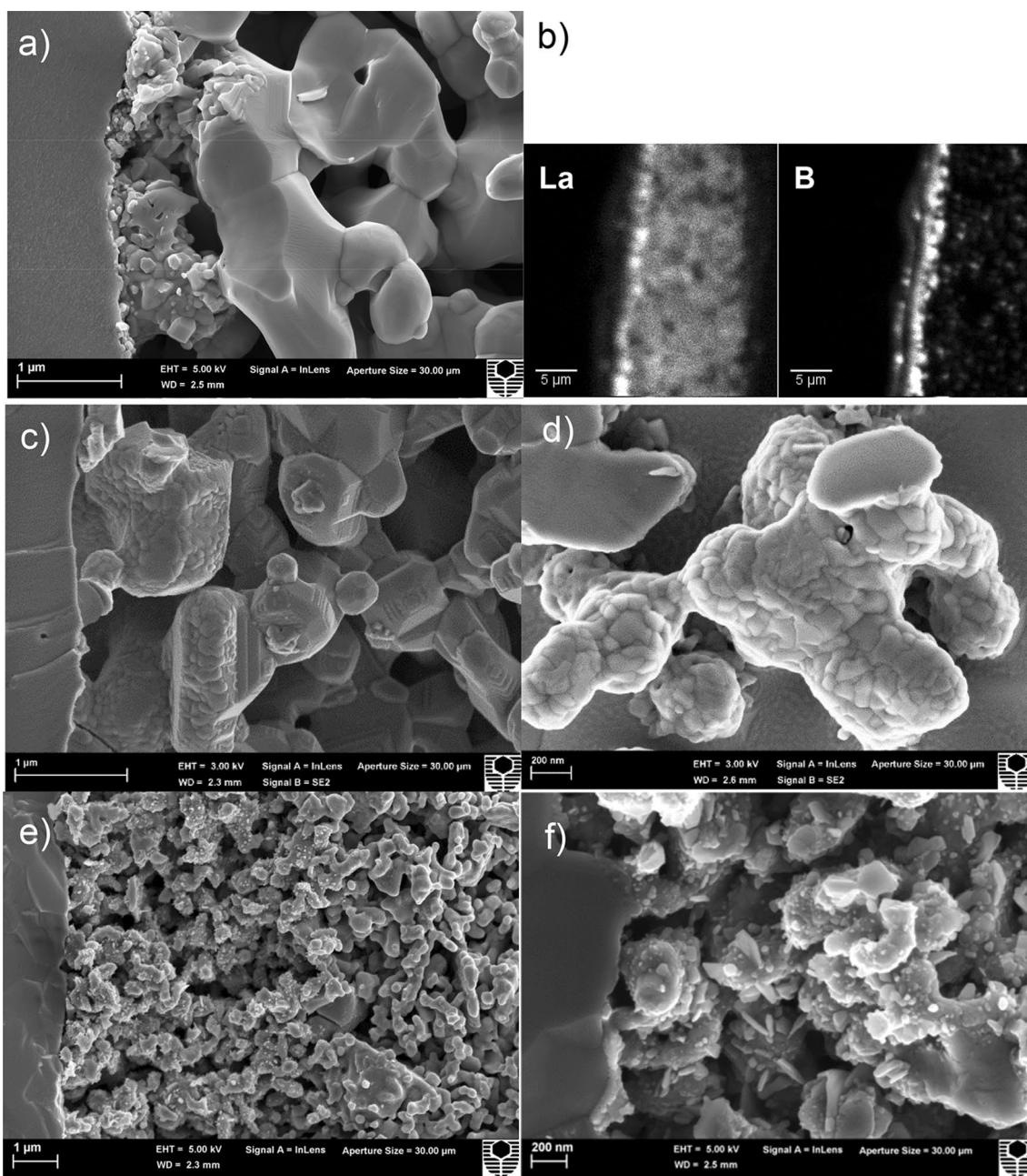
Fig. 15 SEM micrograph and Nano-SIMS imaging of the cross section (a–c) and the exposed YSZ electrolyte surface (d) of LSM electrodes after polarization in the presence of borosilicate glass; (a, b) after cathodic polarization at 0.2 \text{ A cm}^{-2} and 800 \text{ }^\circ\text{C} for 100 h; (c, d) after anodic polarization at 0.050 \text{ A cm}^{-2} and 800 \text{ }^\circ\text{C} for 8 h; and (e,
