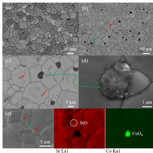
Fig. 4 SEM micrographs of a freshly prepared LSCF and b LSCF after heat treatment at 800 °C in air for 96 h; c , d enlarged images of the segregated micron-sized particles and e EDS element mapping of Sr and Co. Arrows indicate segregated and isolated submicron-sized particles and large particles, modified based on Ref. [86]. Reproduced with permission from Ref. [86]. Copyright 2014, Royal Society of Chemistry
