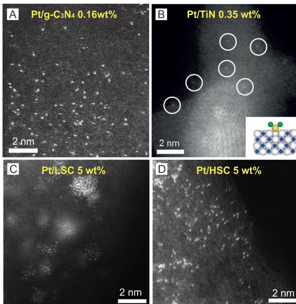
Fig. 1 HAADF-STEM images of Pt single atoms on different substrates: a g-C 3 N 4 , b TiN, c LSC, d HSC. a Adapted with permission from Ref. [19]. Copyright 2016, Wiley-VCH. b Adapted with permission from Ref. [20]. Copyright 2016, Wiley-VCH. c , d Adapted with permission from Ref. [22]. Copyright 2016, Nature Publishing Group
