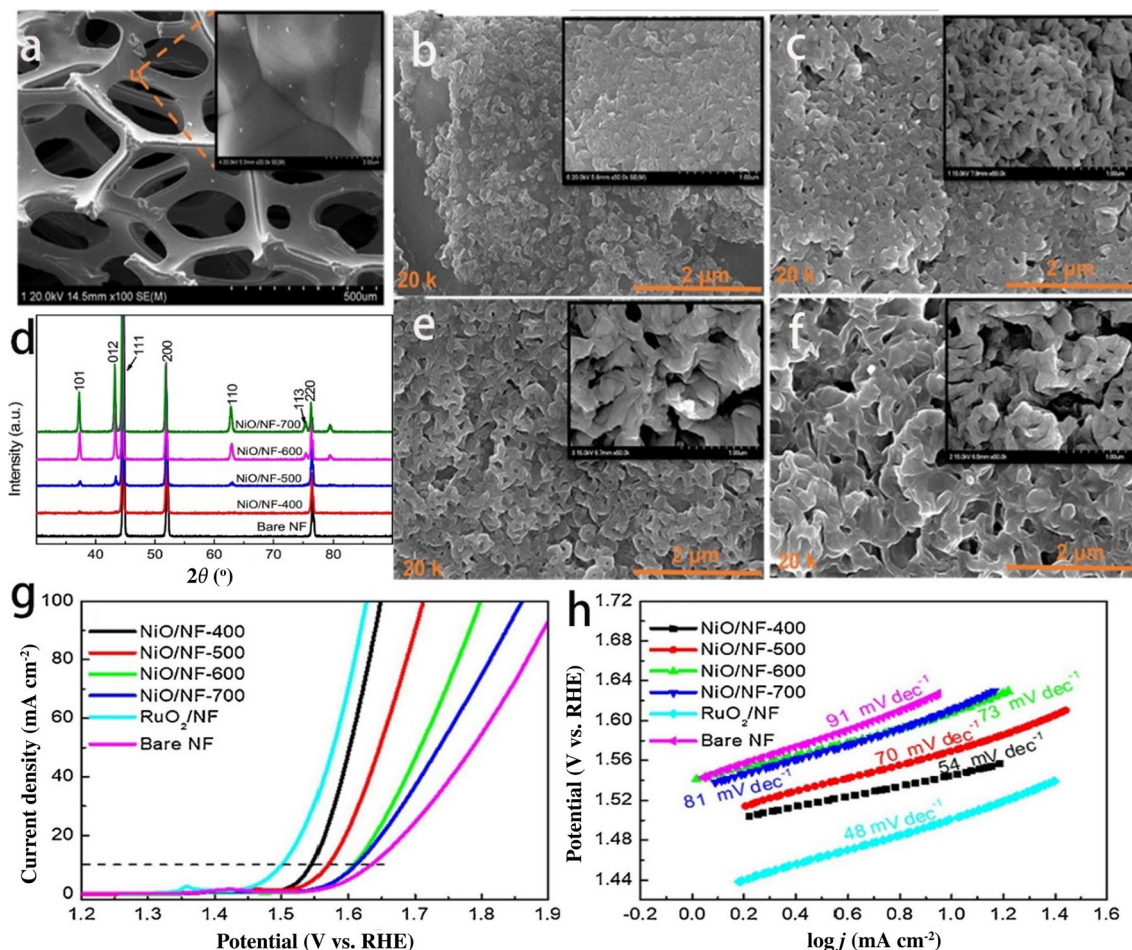
Fig. 4 a–f XRD pattern of NiO/NF and SEM images at different temperatures. g OER polarization curves. h Tafel plots [63]
