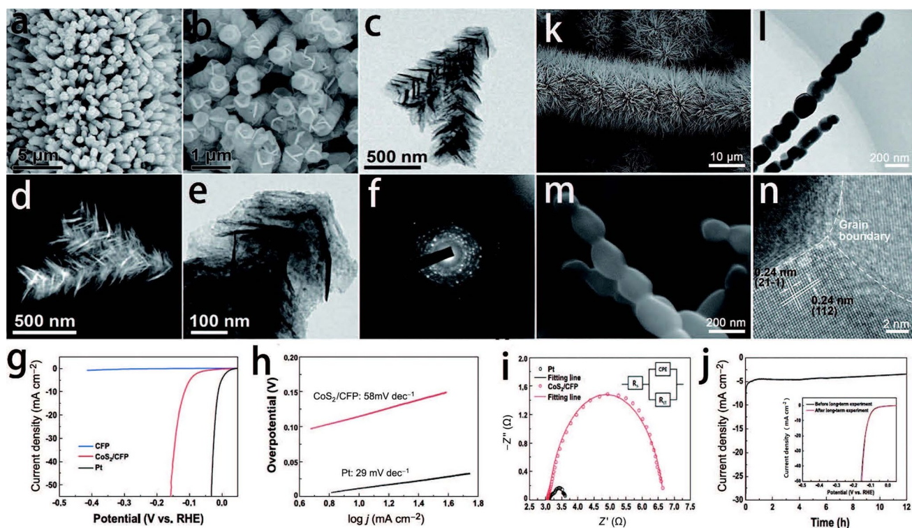
Fig. 20 a–f SEM, TEM and SAED patterns of CoS 2 nanopine tree array. g–j Polarization curve, Tafel slope, EIS spectra and long-term stability test of CoS 2 [300]. k–n SEM images and TEM images of the necklace-like CoS 2 NWs on CFP (selenized at 450 °C) [302]
