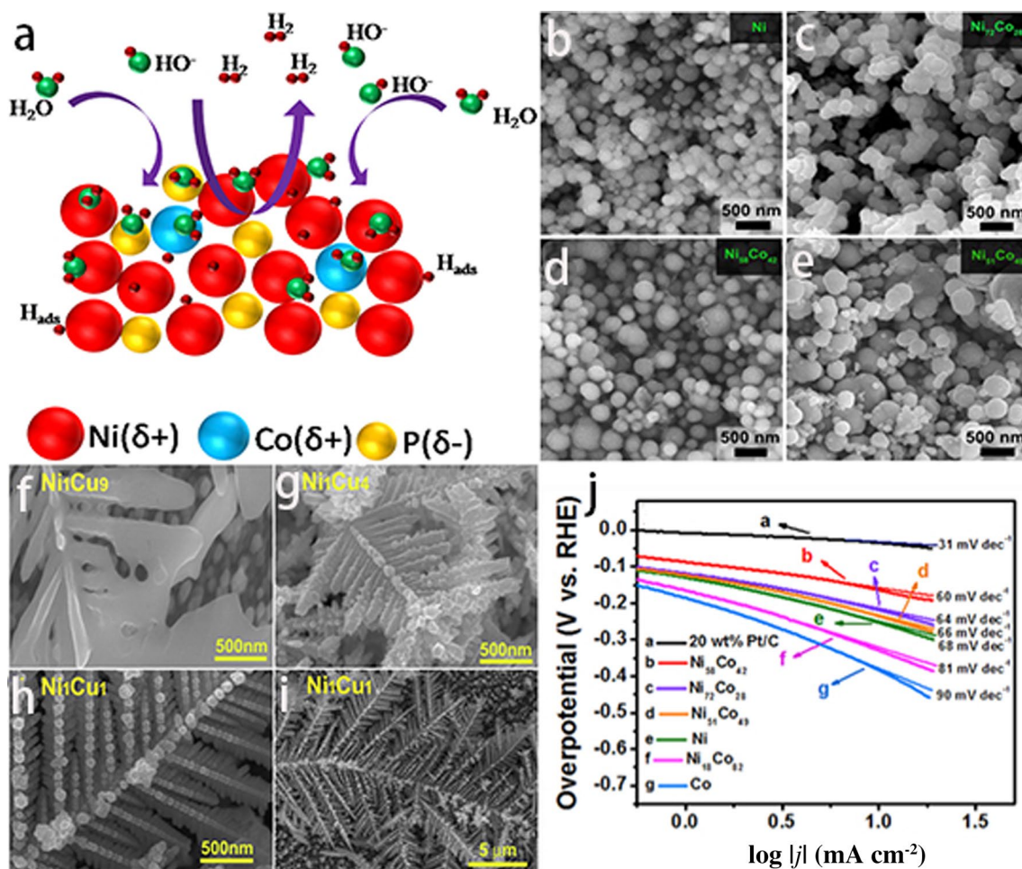
Fig. 16 a Schematic illustration of electrocatalytic HER on the surface of catalysts in alkaline media [248]. b–e SEM images of mesostructured Ni_{100-x}Co_x alloys prepared from different LLC compositions.
