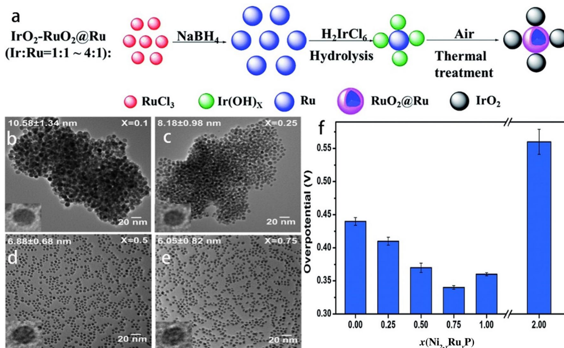
Fig. 3 a Schematic illustration of the synthesis of \text{IrO}_2\text{-RuO}_2\text{@Ru} nanocatalysts [58]. b–e TEM images for \text{Ni}_{2-x}\text{Ru}_x\text{P} nanoparticles. f Changes in overpotential (at 10\text{ mA cm}^{-2} ) for different compositions of \text{Ni}_{2-x}\text{Ru}_x\text{P} in 1.0 M KOH [59]
